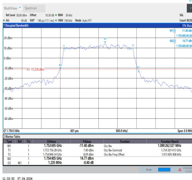
Band4-1.4MHz-64QAM-20393-6RB#0-PASS
