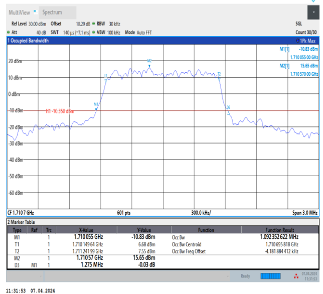
Band4-1.4MHz-16QAM-19957-6RB#0-PASS
