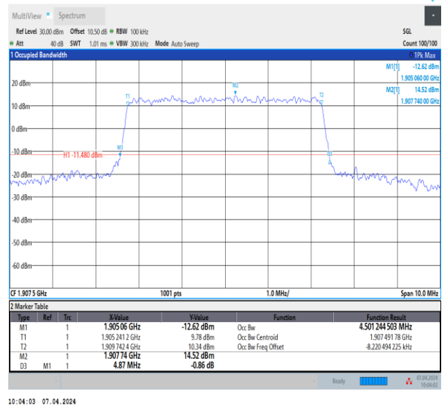
Band2-5MHz-16QAM-19175-25RB#0-PASS
