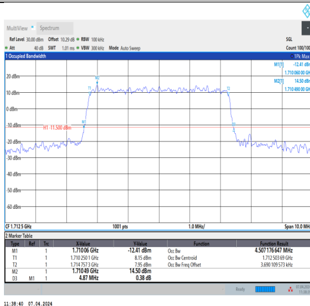
Band4-5MHz-64QAM-19975-25RB#0-PASS
