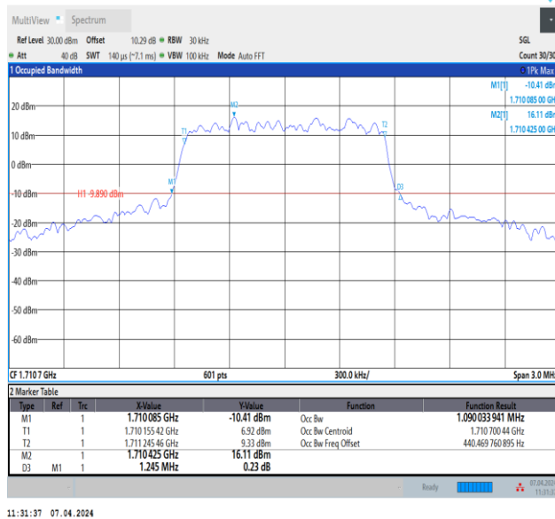
Band4-1.4MHz-QPSK-19957-6RB#0-PASS
