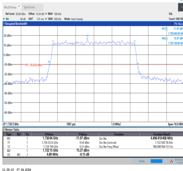
Band4-5MHz-16QAM-20175-25RB#0-PASS
