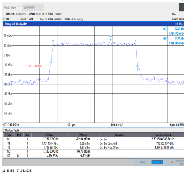
Band4-3MHz-QPSK-20175-15RB#0-PASS
