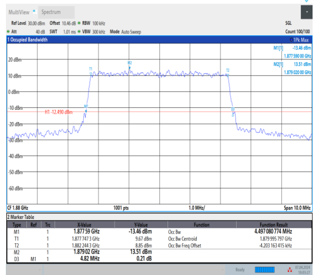
Band2-5MHz-64QAM-18900-25RB#0-PASS
