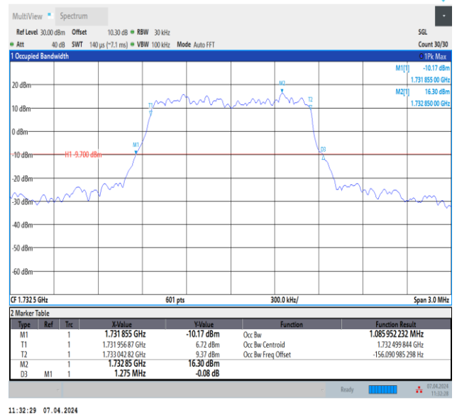
Band4-1.4MHz-QPSK-20175-6RB#0-PASS
