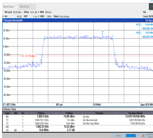
Band2-15MHz-64QAM-18675-75RB#0-PASS
