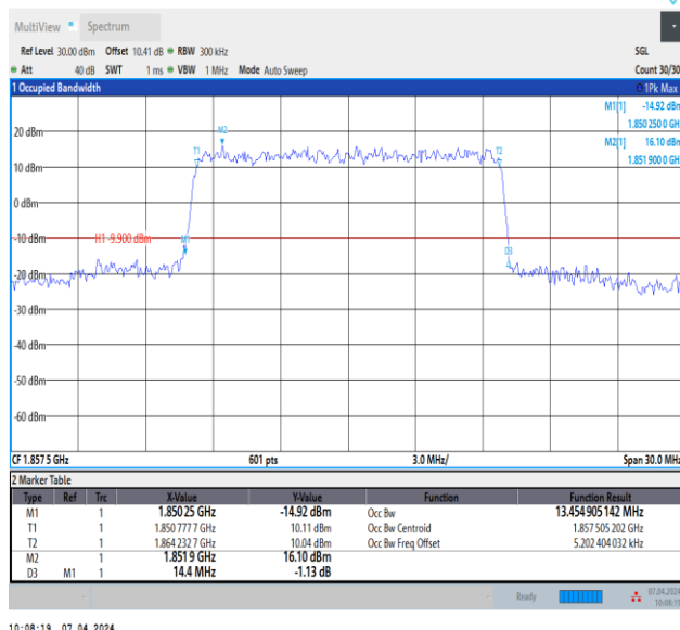
Band2-15MHz-QPSK-18675-75RB#0-PASS
