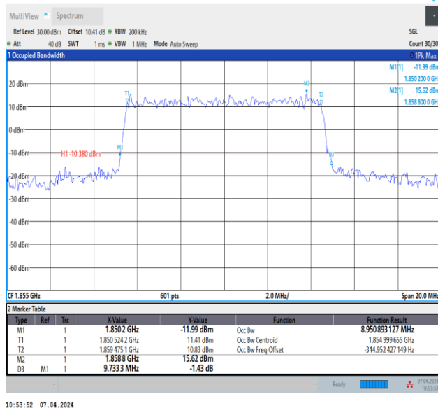
Band2-10MHz-16QAM-18650-50RB#0-PASS
