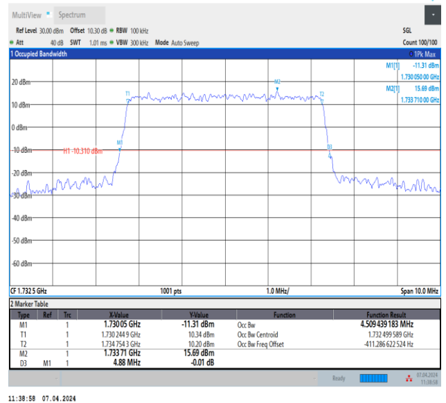
Band4-5MHz-QPSK-20175-25RB#0-PASS
