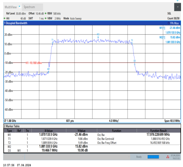
Band2-20MHz-16QAM-18900-100RB#0-PASS
