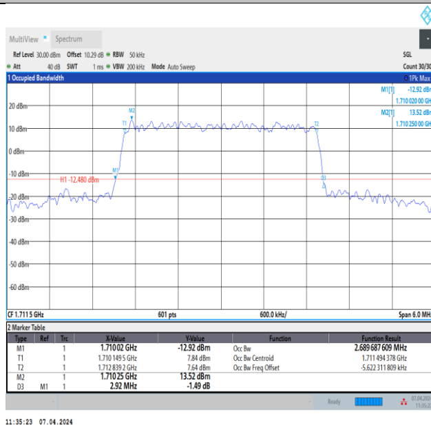
Band4-3MHz-16QAM-19965-15RB#0-PASS
