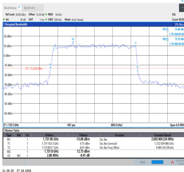
Band4-3MHz-64QAM-20175-15RB#0-PASS
