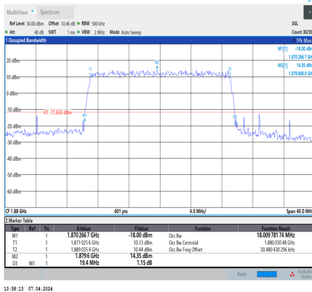
Band2-20MHz-64QAM-18900-100RB#0-PASS
