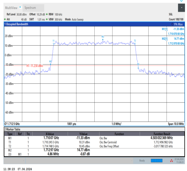
Band4-5MHz-16QAM-19975-25RB#0-PASS
