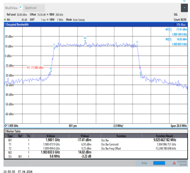
Band2-10MHz-64QAM-19150-50RB#0-PASS
