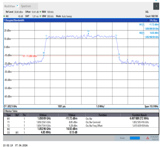
Band2-5MHz-16QAM-18625-25RB#0-PASS
