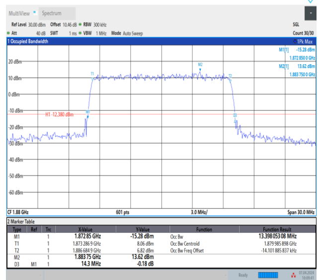
Band2-15MHz-64QAM-18900-75RB#0-PASS
