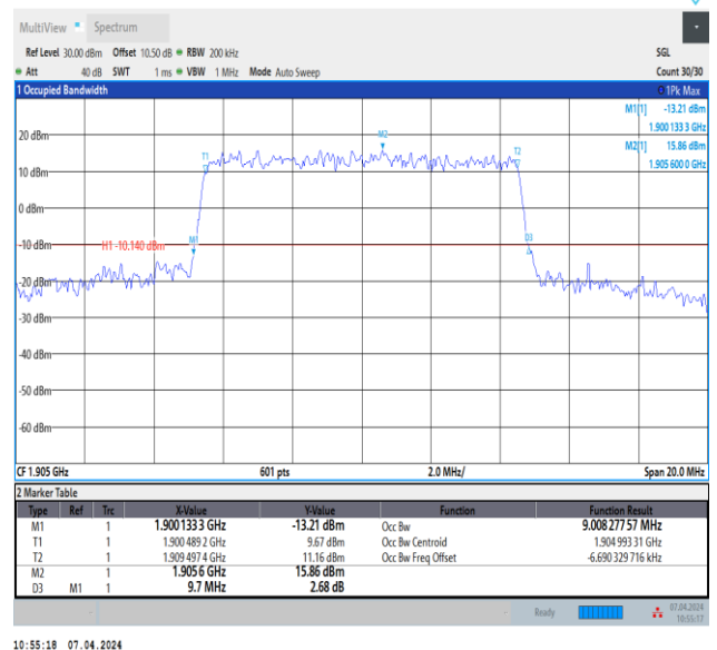
Band2-10MHz-QPSK-19150-50RB#0-PASS
