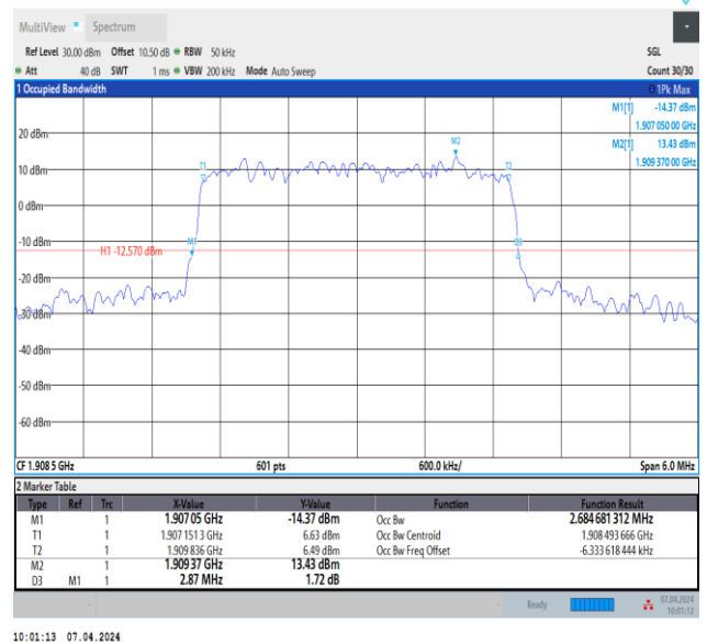
Band2-3MHz-64QAM-19185-15RB#0-PASS
