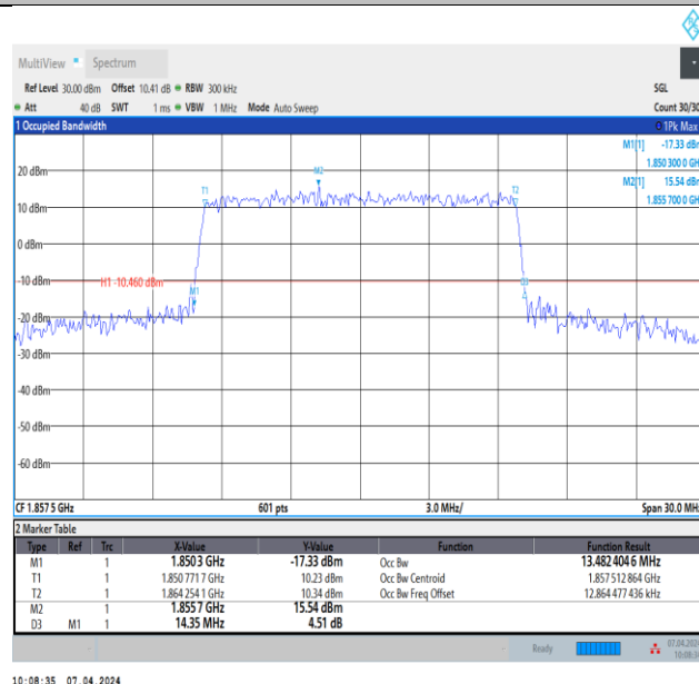
Band2-15MHz-16QAM-18675-75RB#0-PASS
