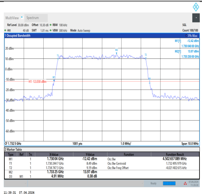
Band4-5MHz-64QAM-20175-25RB#0-PASS
