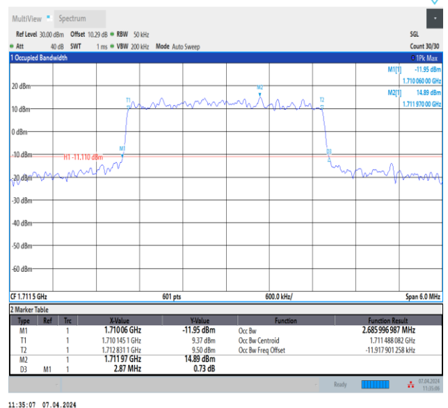
Band4-3MHz-QPSK-19965-15RB#0-PASS
