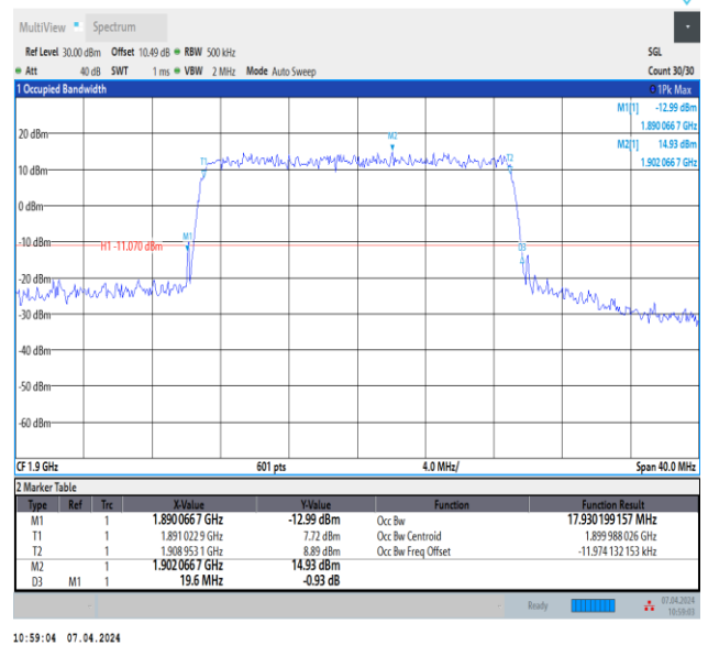
Band2-20MHz-64QAM-19100-100RB#0-PASS
