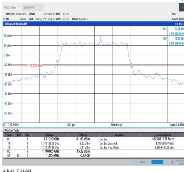
Band4-1.4MHz-64QAM-19957-6RB#0-PASS
