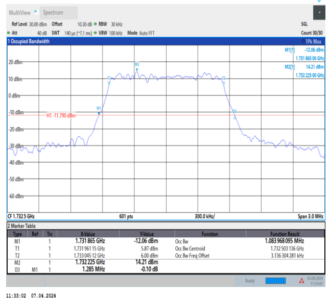
Band4-1.4MHz-64QAM-20175-6RB#0-PASS
