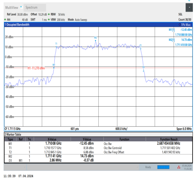
Band4-3MHz-64QAM-19965-15RB#0-PASS
