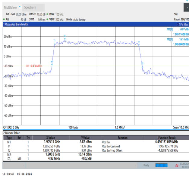
Band2-5MHz-QPSK-19175-25RB#0-PASS
