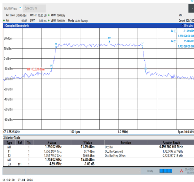
Band4-5MHz-QPSK-20375-25RB#0-PASS
