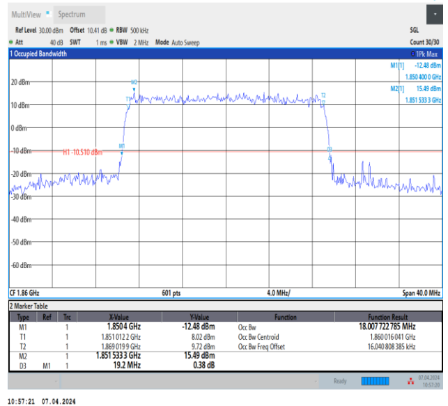
Band2-20MHz-64QAM-18700-100RB#0-PASS
