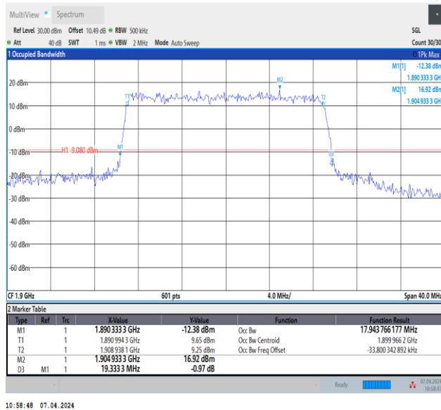
Band2-20MHz-16QAM-19100-100RB#0-PASS
