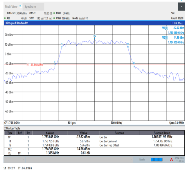
Band4-1.4MHz-16QAM-20393-6RB#0-PASS
