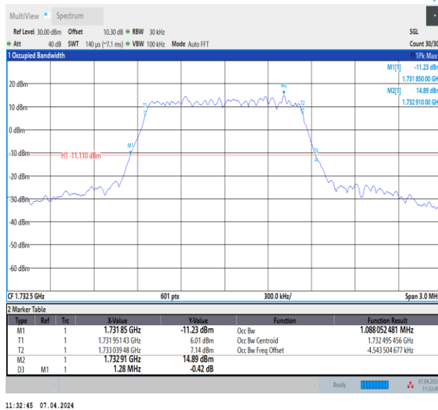
Band4-1.4MHz-16QAM-20175-6RB#0-PASS
