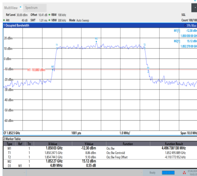
Band2-5MHz-64QAM-18625-25RB#0-PASS
