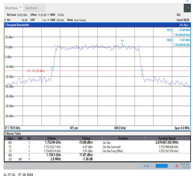
Band4-3MHz-64QAM-20385-15RB#0-PASS
