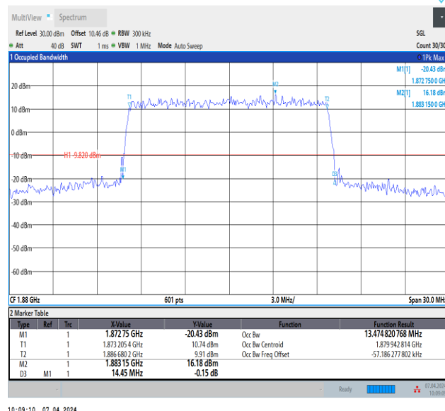
Band2-15MHz-QPSK-18900-75RB#0-PASS
