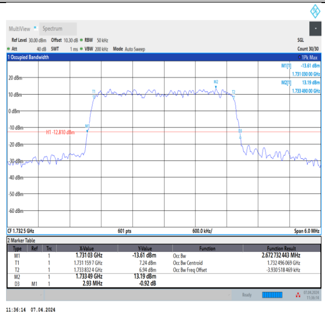
Band4-3MHz-16QAM-20175-15RB#0-PASS
