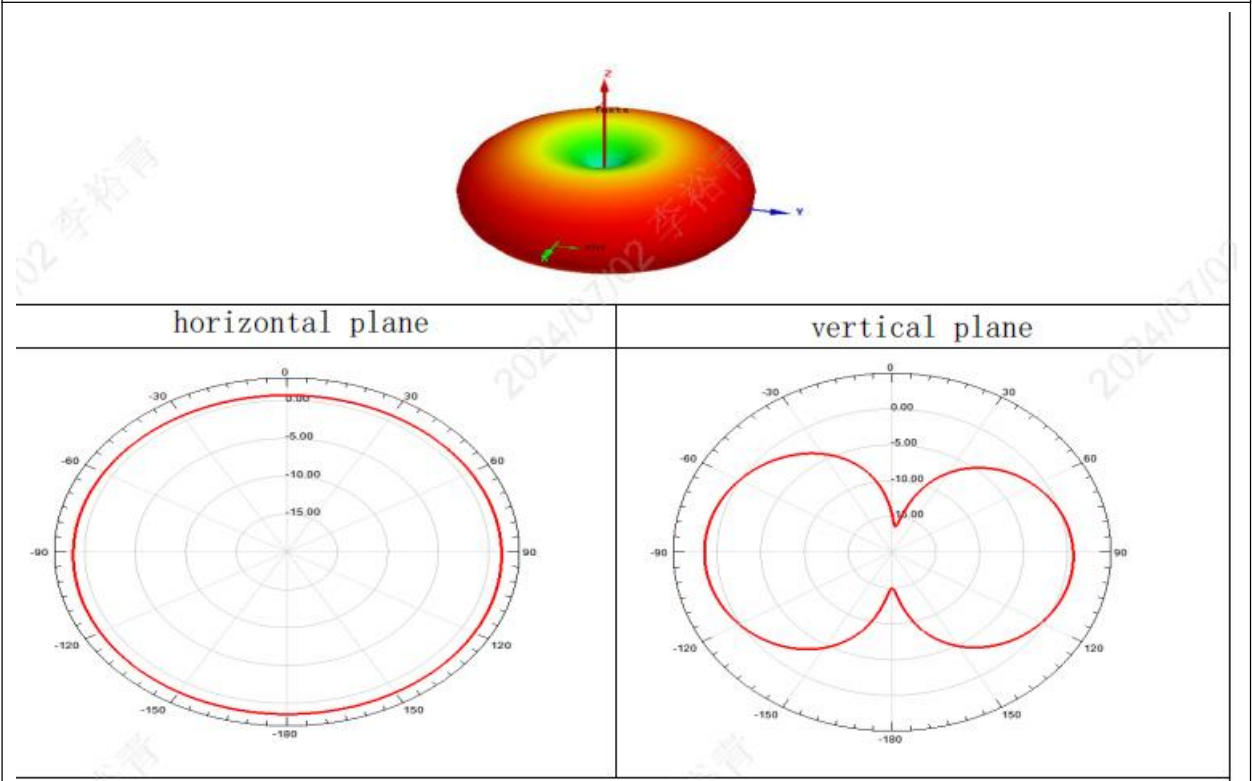
Radiation pattern5.8G
