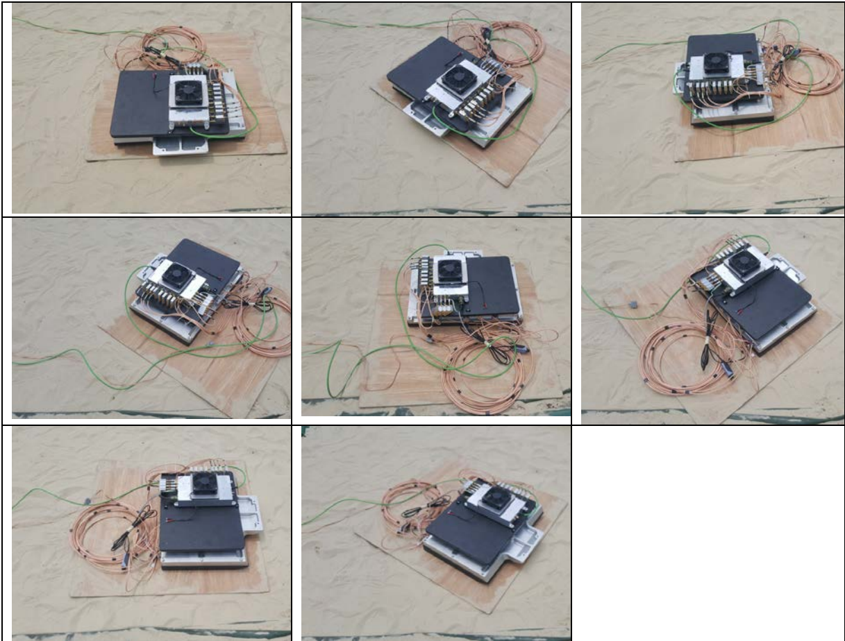
EUT Positions with 45 Degree Interval
