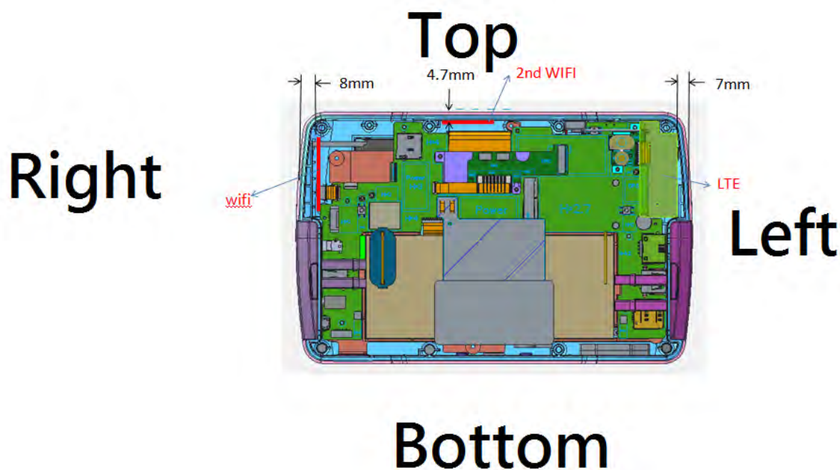
Fig.13 Antenna position of EUT (Back view)
