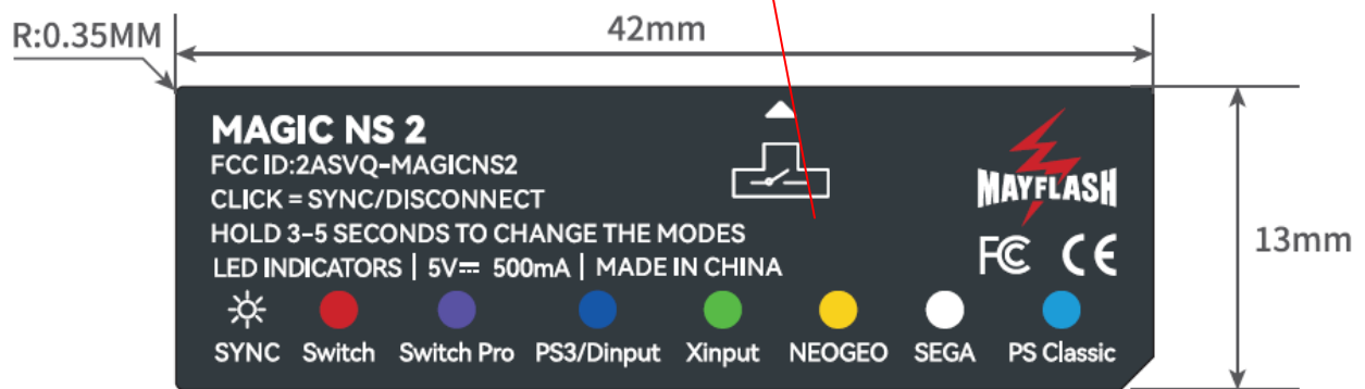
Label Location
