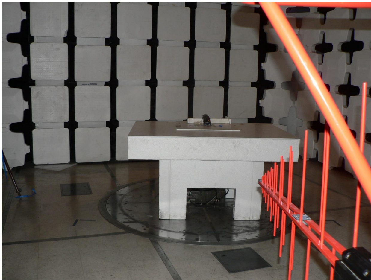
LYFT14 eBike Digital Emissions 30MHz-1000MHz
