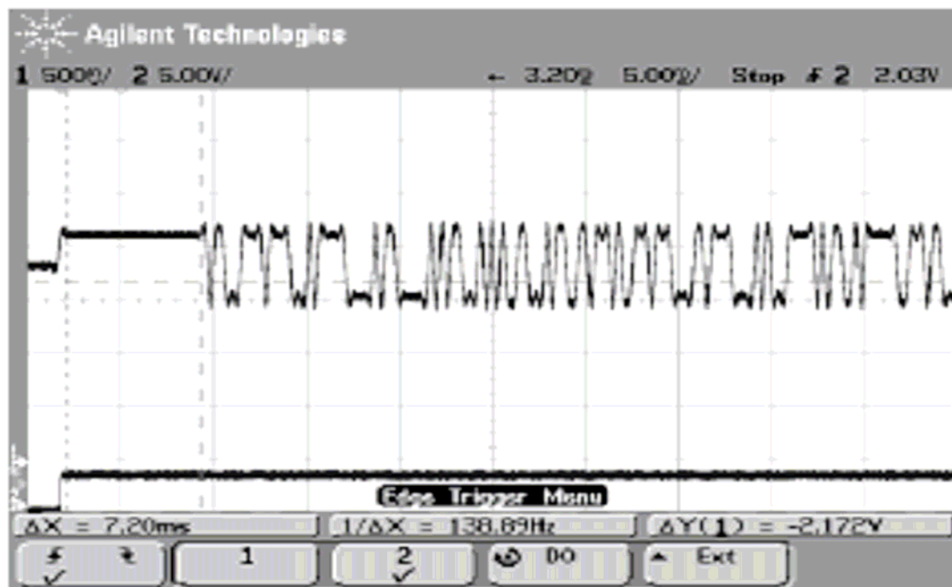
Figure 1. Modulating signal
