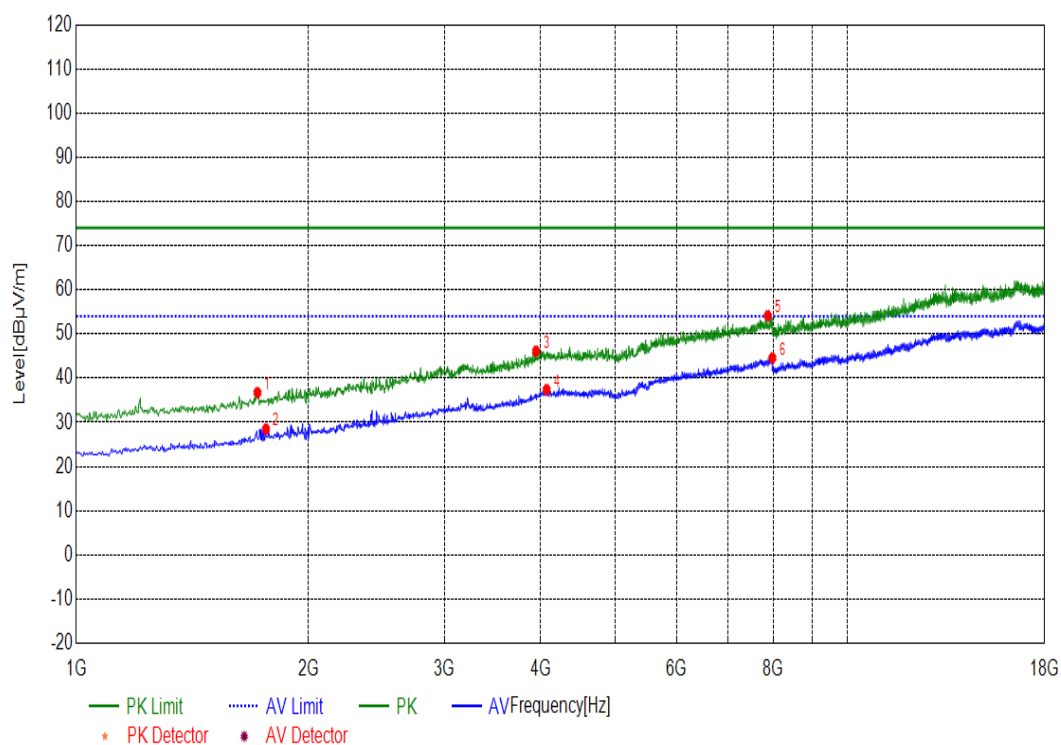
(Plot N: Test Antenna Vertical 1G – 18G)
