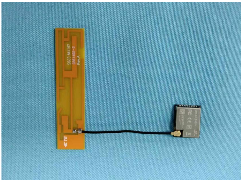
EUT –With Antenna View
