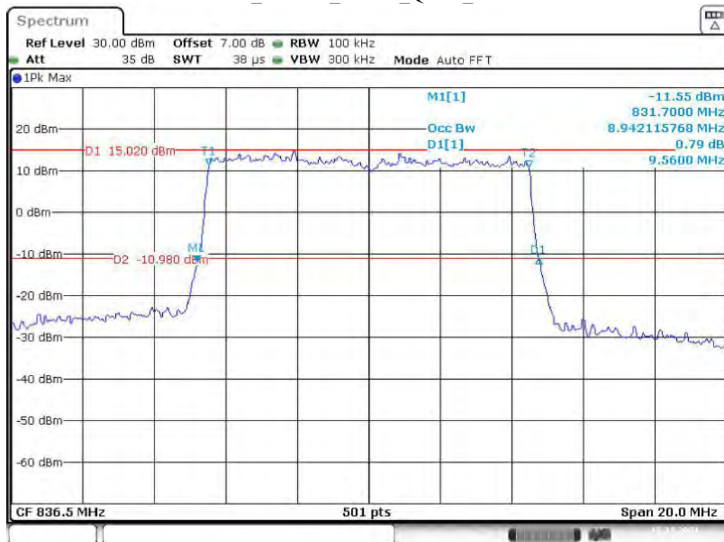
Band 5_10 MHz_Middle_QPSK_RB50#0
