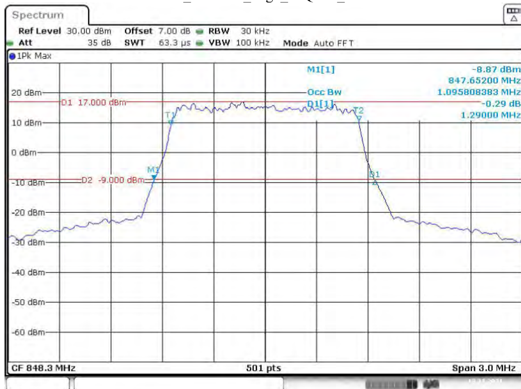
Band 5 1.4 MHz High 16QAM RB6#0
