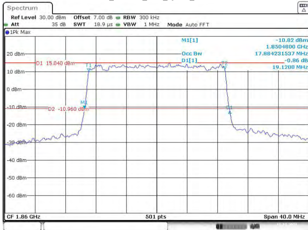
Band 2_20 MHz_Low_QPSK_RB100#0
