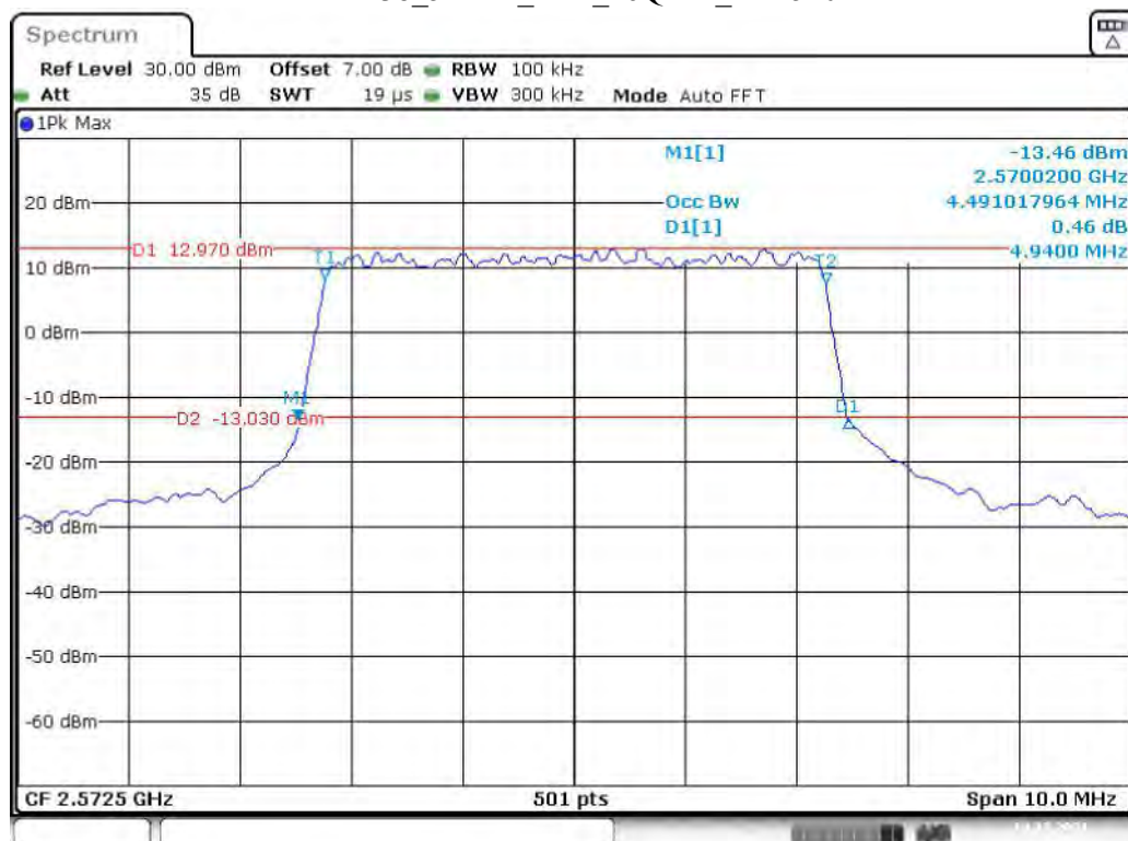
Band 38_5 MHz_Low_16QAM_RB25#0
