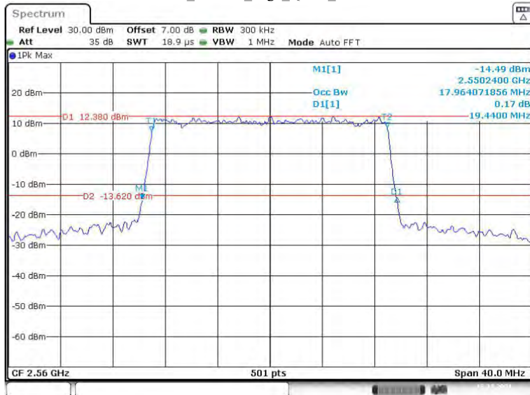
Band 7_20 MHz_High_QPSK_RB100#0
