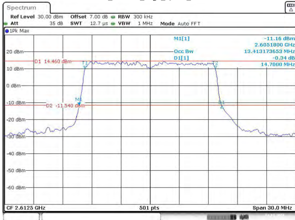
Band 38_15 MHz_High_QPSK_RB75#0
