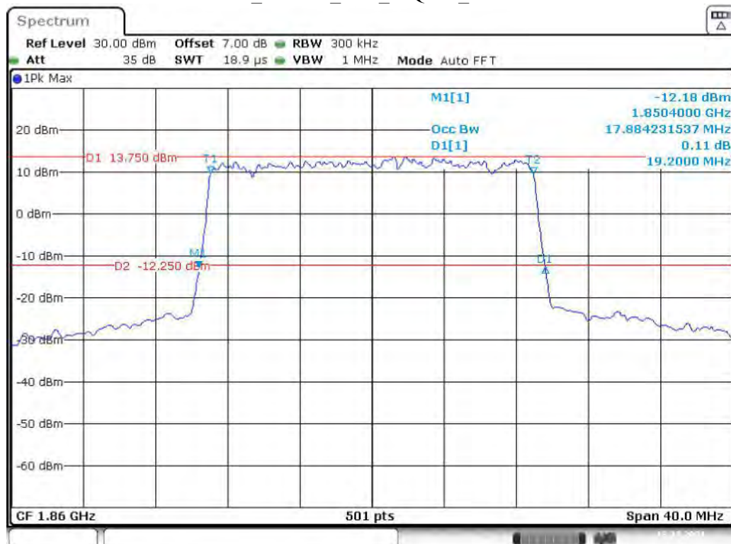
Band 2_20 MHz_Low_16QAM_RB100#0
