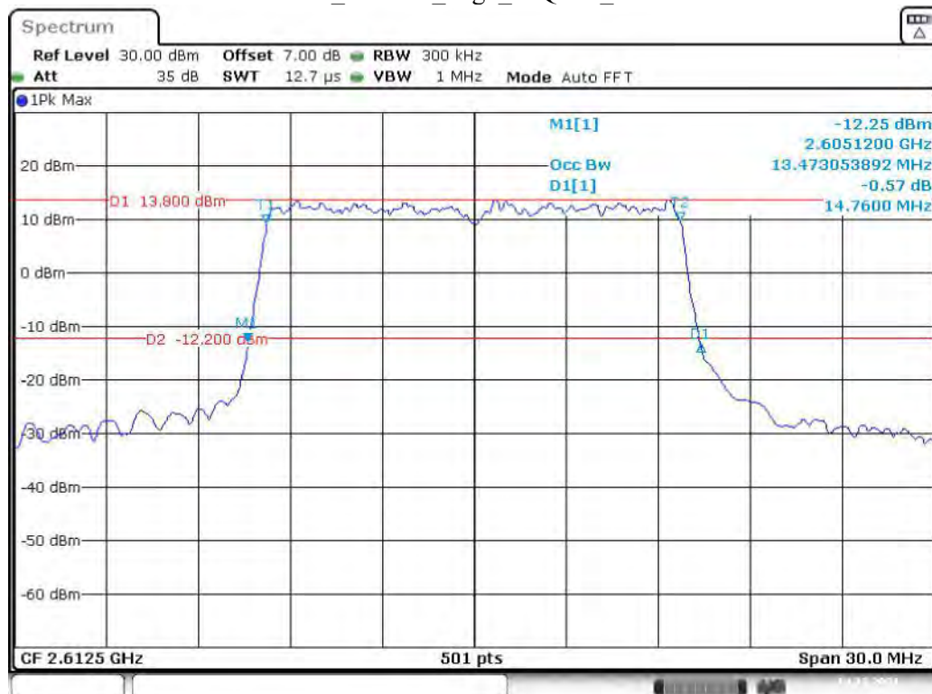
Band 38_15 MHz_High_16QAM_RB75#0
