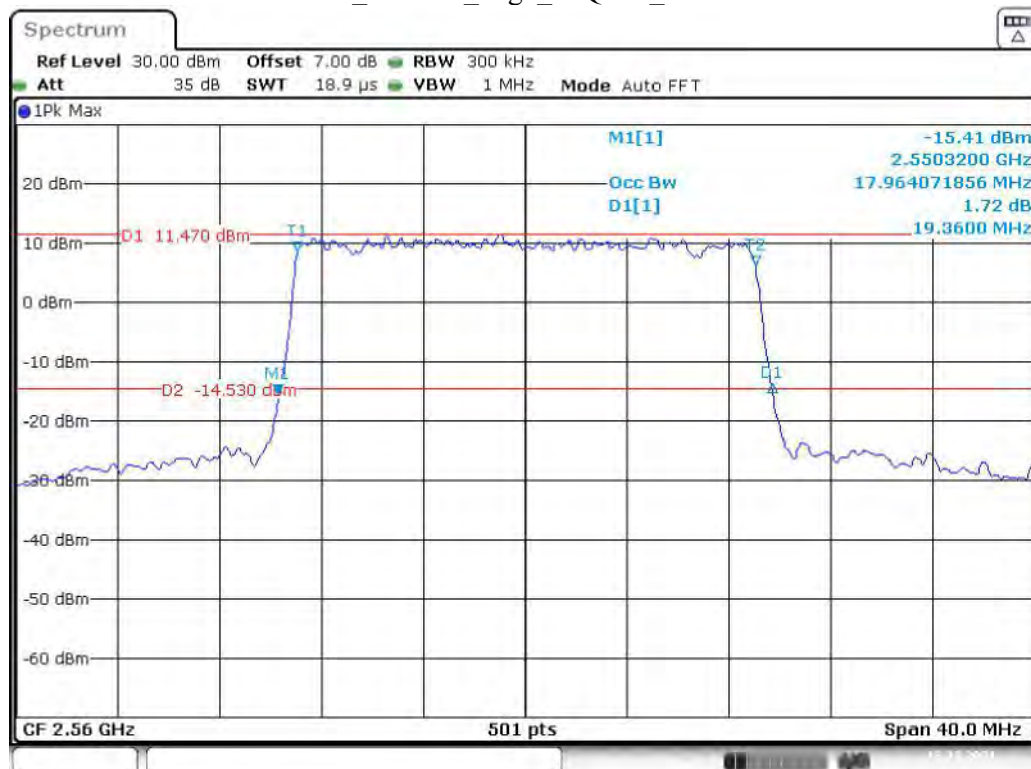
Band 7 20 MHz High 16QAM RB100#0
