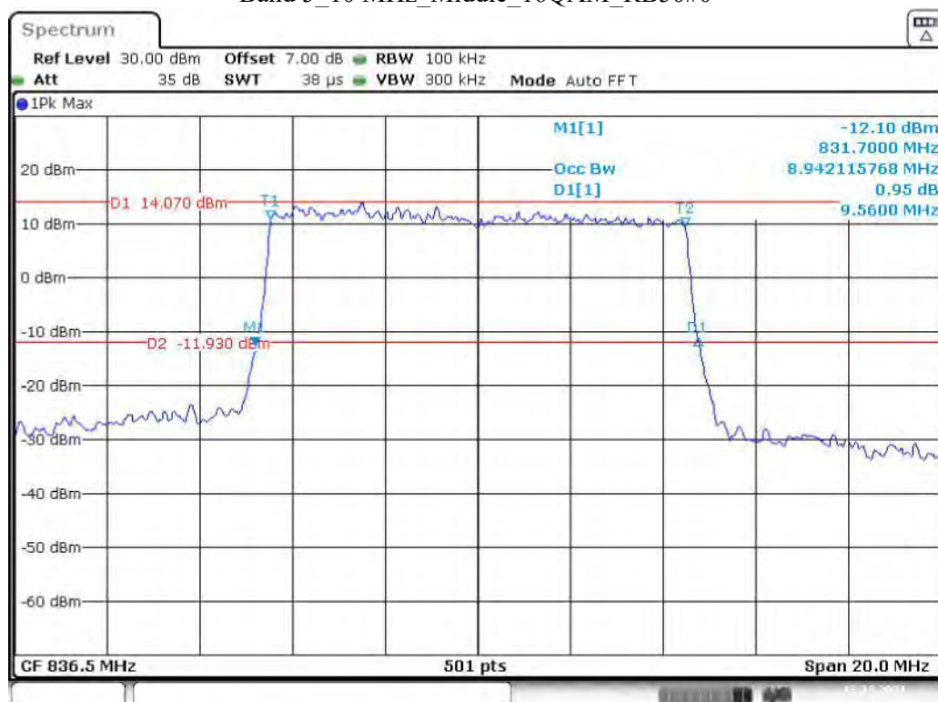
Band 5 10 MHz Middle 16QAM RB50#0
