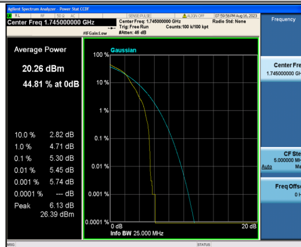
Band4-20MHz-16QAM-20300-1RB#0-PASS
