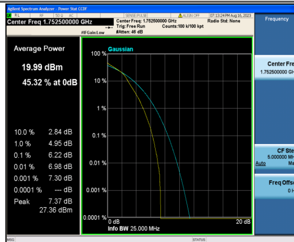
Band4-5MHz-16QAM-20375-25RB#0-PASS
