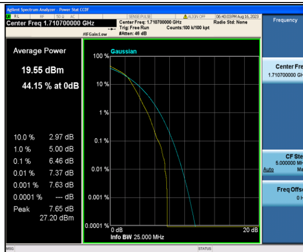
Band4-1.4MHz-16QAM-19957-6RB#0-PASS
