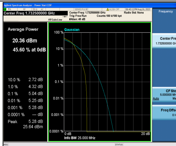
Band4-1.4MHz-16QAM-20175-1RB#0-PASS
