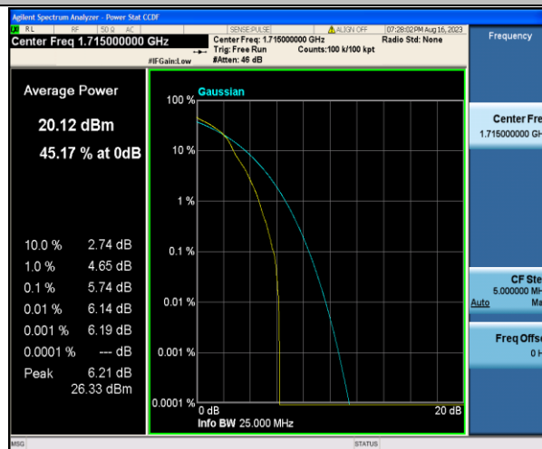
Band4-10MHz-16QAM-20000-1RB#0-PASS
