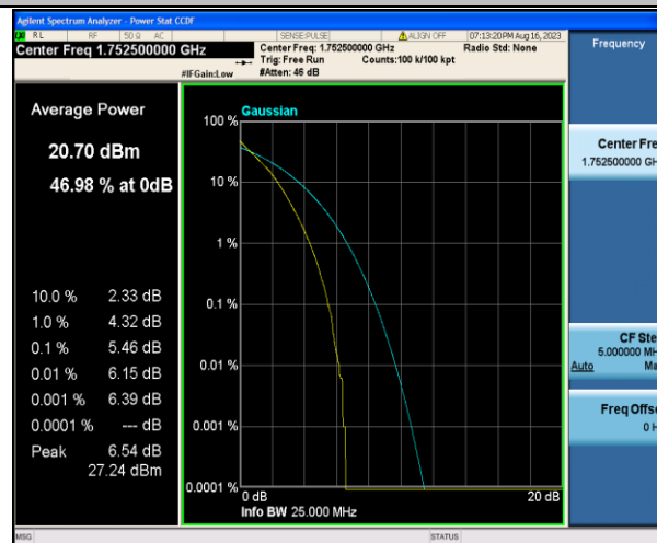
Band4-5MHz-QPSK-20375-25RB#0-PASS
