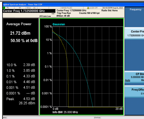
Band4-1.4MHz-QPSK-20175-1RB#0-PASS
