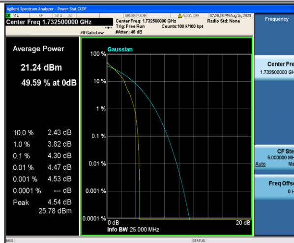
Band4-10MHz-QPSK-20175-1RB#0-PASS
