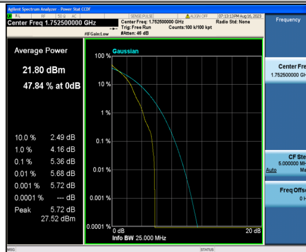
Band4-5MHz-QPSK-20375-1RB#0-PASS
