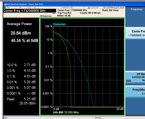
Band4-5MHz-16QAM-20175-1RB#0-PASS
