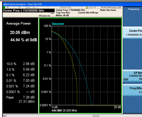
Band4-1.4MHz-16QAM-20393-6RB#0-PASS
