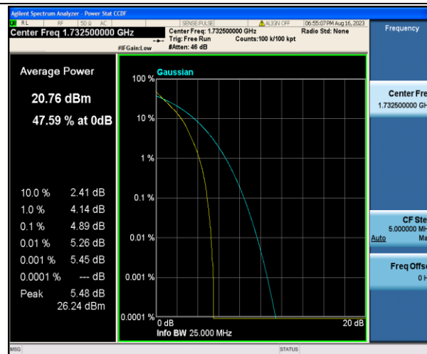
Band4-3MHz-QPSK-20175-15RB#0-PASS
