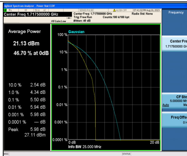
Band4-15MHz-QPSK-20025-1RB#0-PASS
