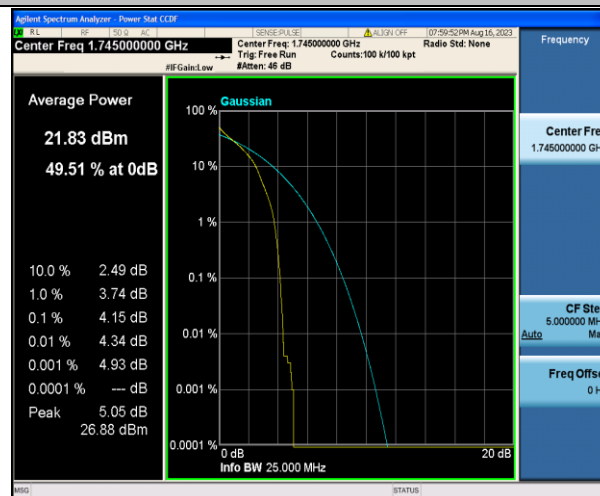
Band4-20MHz-QPSK-20300-1RB#0-PASS
