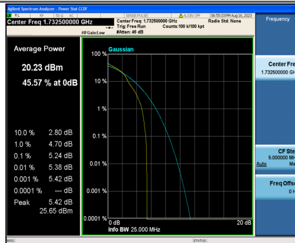
Band4-3MHz-16QAM-20175-1RB#0-PASS
