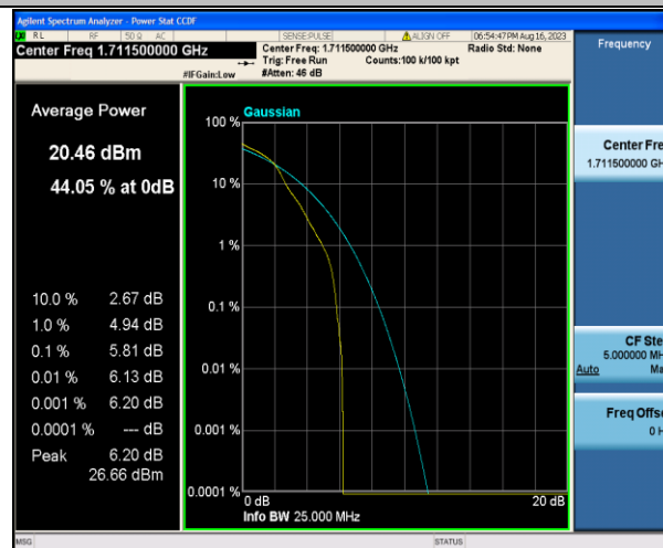
Band4-3MHz-16QAM-19965-1RB#0-PASS
