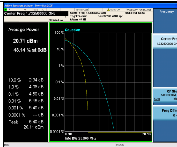
Band4-5MHz-QPSK-20175-25RB#0-PASS
