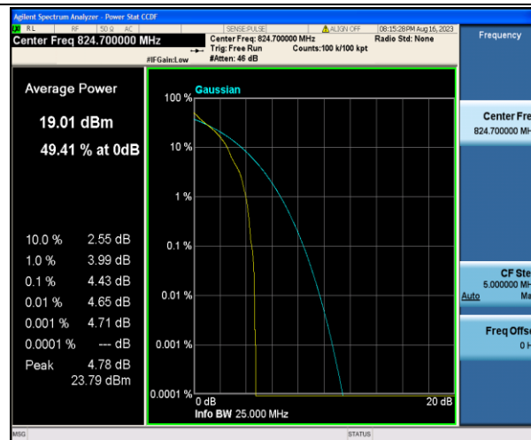
Band5-1.4MHz-QPSK-20407-1RB#0-PASS
