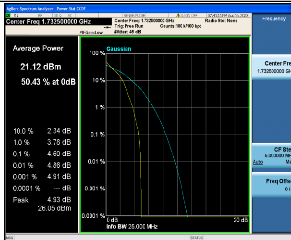
Band4-15MHz-QPSK-20175-1RB#0-PASS
