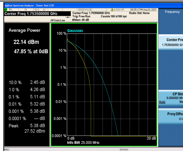
Band4-3MHz-QPSK-20385-1RB#0-PASS
