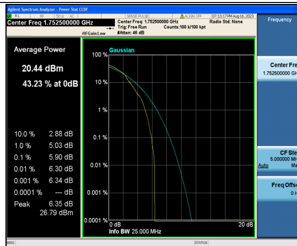
Band4-5MHz-16QAM-20375-1RB#0-PASS
