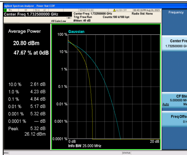
Band4-1.4MHz-QPSK-20175-6RB#0-PASS
