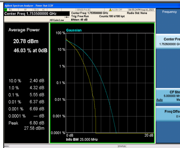
Band4-3MHz-QPSK-20385-15RB#0-PASS
