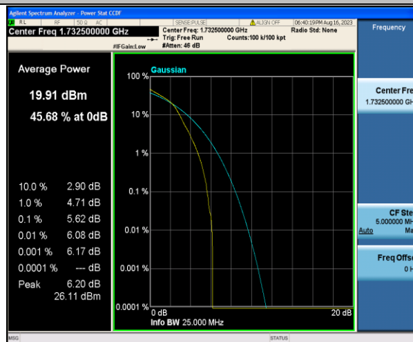
Band4-1.4MHz-16QAM-20175-6RB#0-PASS
