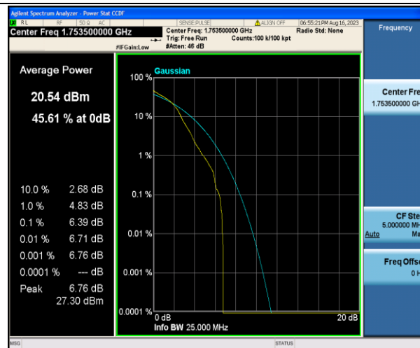
Band4-3MHz-16QAM-20385-1RB#0-PASS
