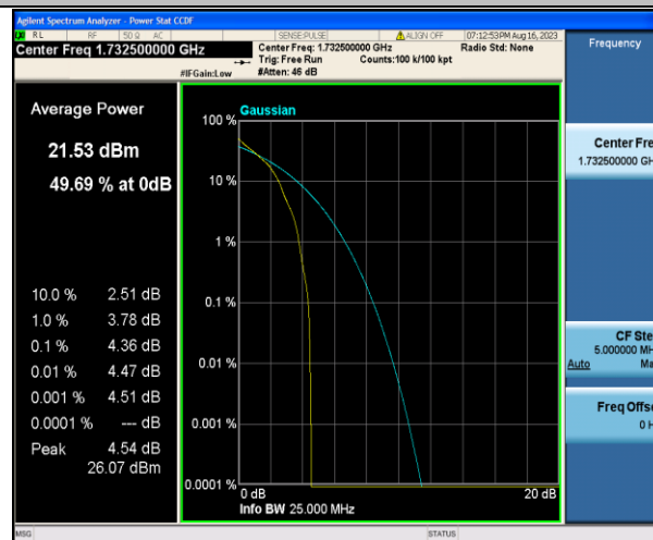
Band4-5MHz-QPSK-20175-1RB#0-PASS
