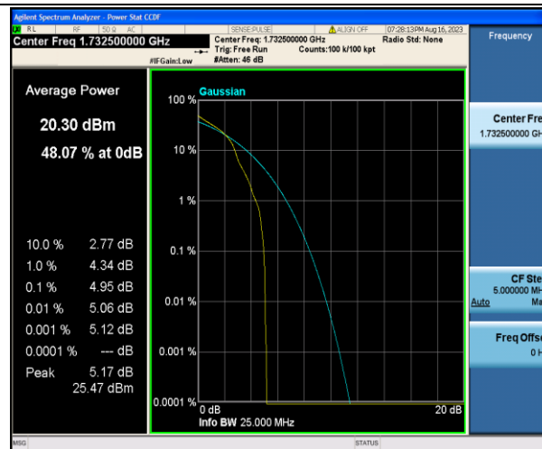
Band4-10MHz-16QAM-20175-1RB#0-PASS
