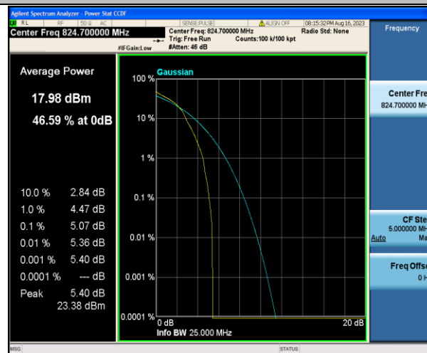
Band5-1.4MHz-16QAM-20407-1RB#0-PASS
