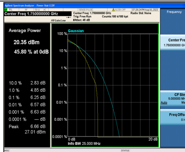
Band4-10MHz-16QAM-20350-1RB#0-PASS
