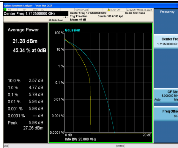
Band4-5MHz-QPSK-19975-1RB#0-PASS
