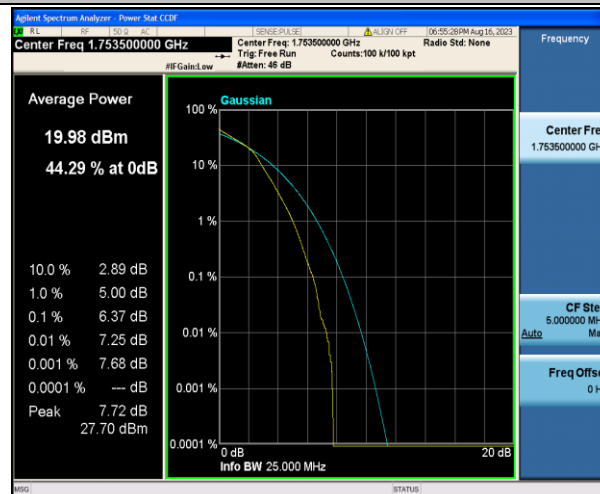
Band4-3MHz-16QAM-20385-15RB#0-PASS
