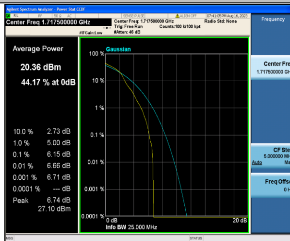
Band4-15MHz-16QAM-20025-1RB#0-PASS
