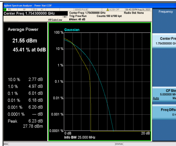
Band4-1.4MHz-16QAM-20393-1RB#0-PASS
