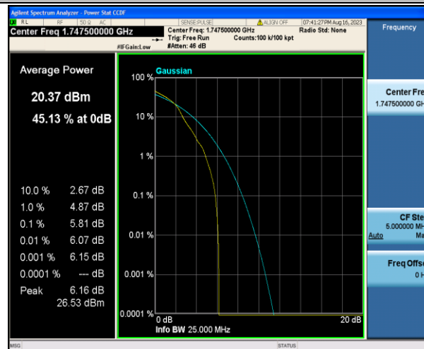
Band4-15MHz-16QAM-20325-1RB#0-PASS
