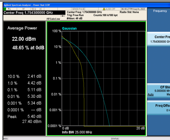
Band4-1.4MHz-QPSK-20393-1RB#0-PASS
