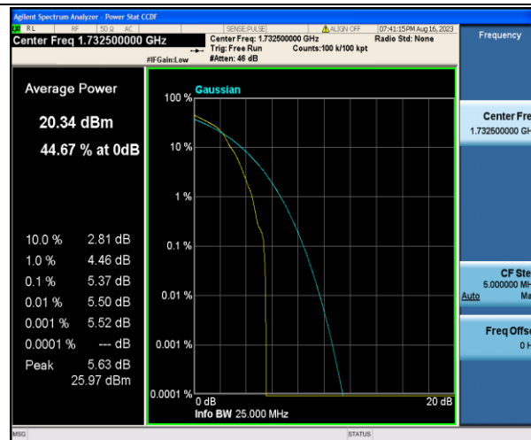
Band4-15MHz-16QAM-20175-1RB#0-PASS
