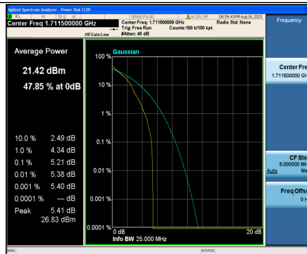
Band4-3MHz-QPSK-19965-1RB#0-PASS
