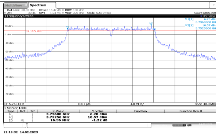
11A-CDD_Ant4_5745
