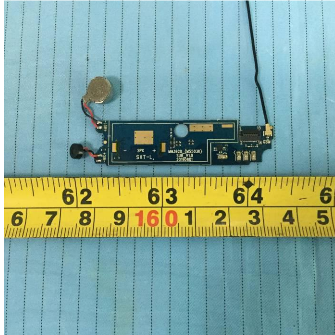
EUT –Small Board Bottom View
