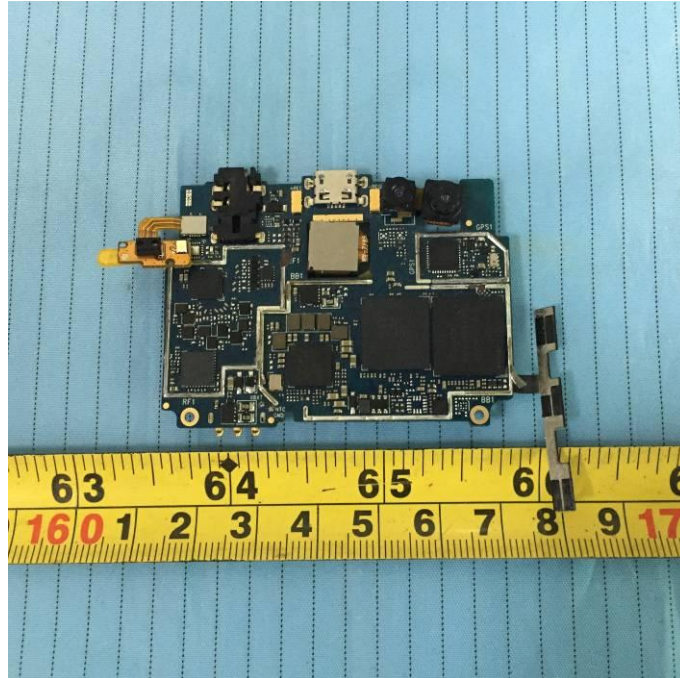
EUT –Main Board Bottom Shieding off View
