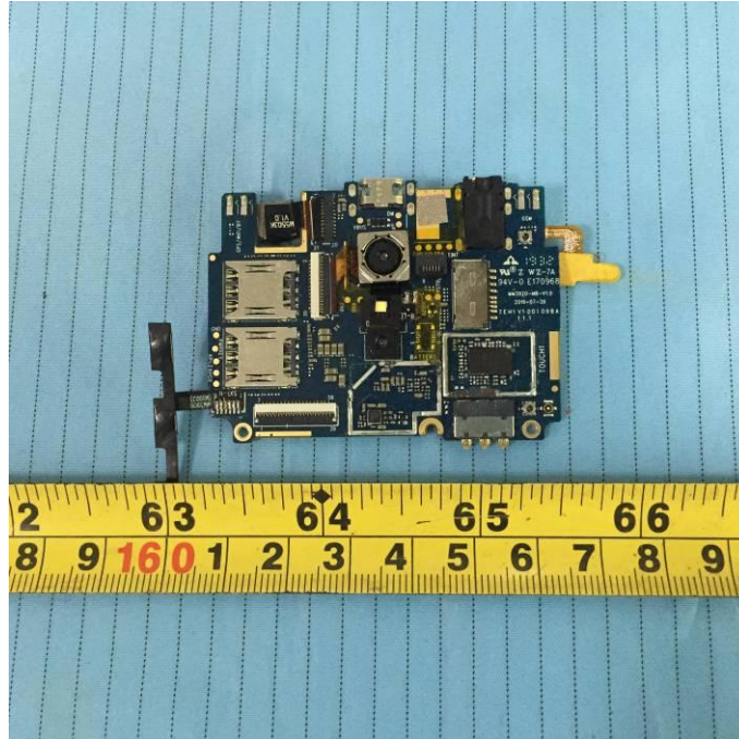
EUT – Main Board Top Shielding off View
