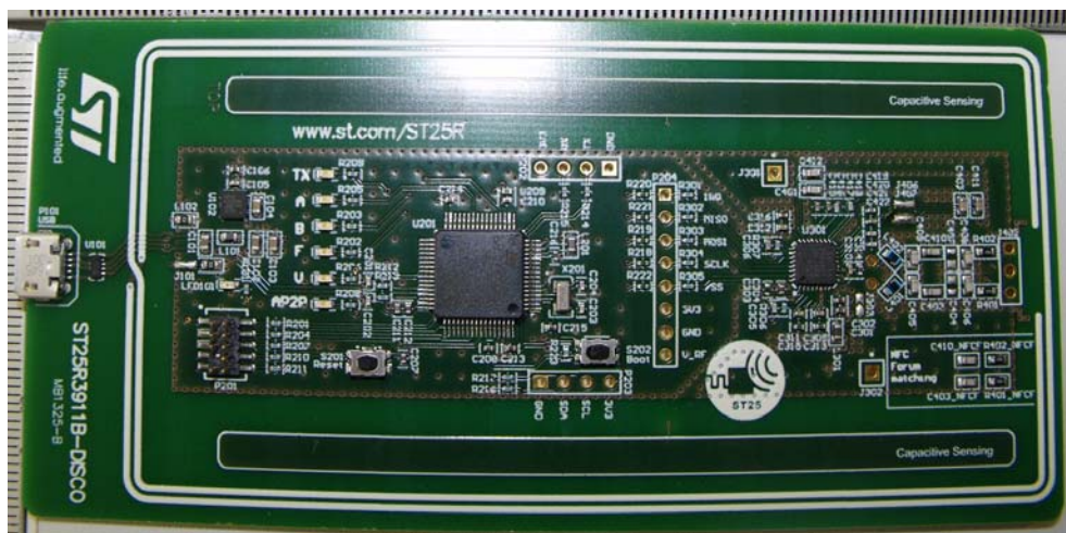
Figure 2: Reader board HF NFC– Top side
