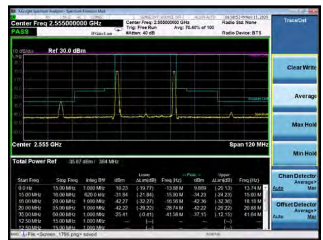
CA_7C 64QAM 20MHz+10MHz CH-High, 100%RB
