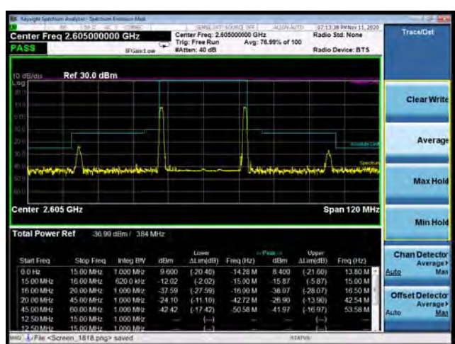
CA_38C 16QAM 15MHz+15MHz CH-High, 1 RB
