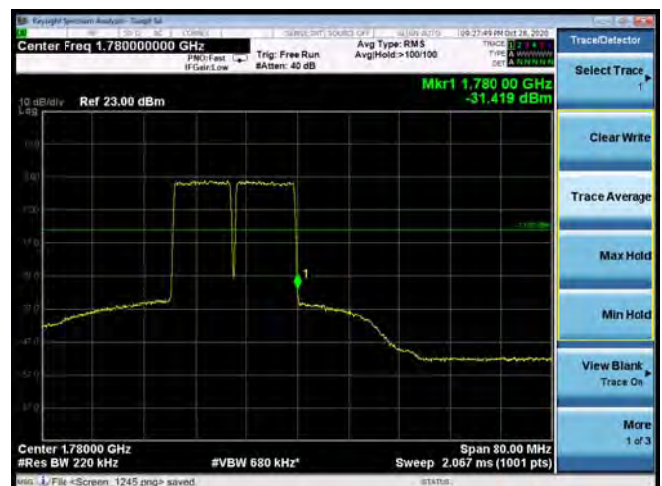
CA_66B 64QAM 10MHz+10MHz CH-High, 100%RB
