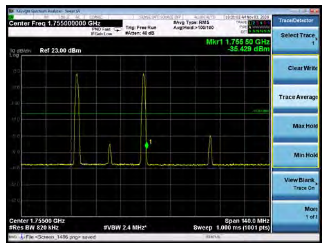
CA-4C-12A 16QAM 20MHz+20MHz+20MHz CH-High, 1 RB
