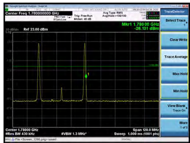
CA_66C 64QAM 20MHz+20MHz CH-High, 100%RB
