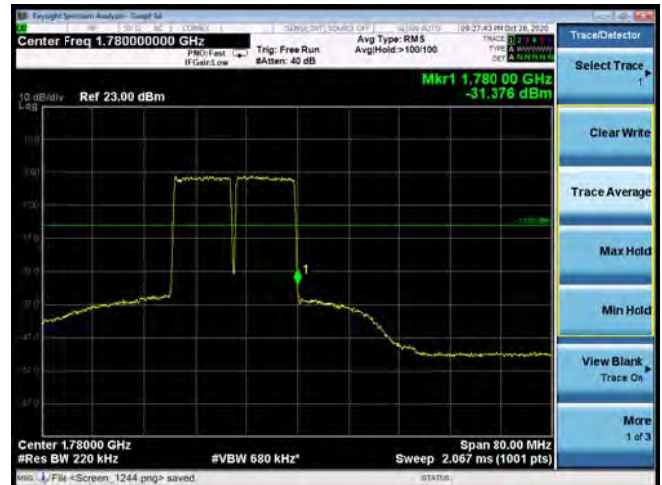
CA_66B 64QAM 10MHz+10MHz CH-High, 1 RB
