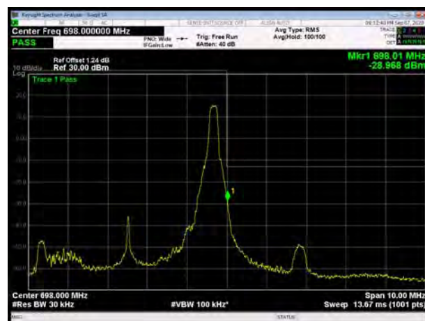
LTE Band 71 64QAM 5MHz CH-High, 100%RB
