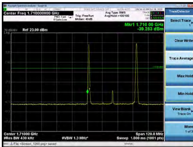
CA_66C 64QAM 20MHz+20MHz CH-Low, 100%RB
