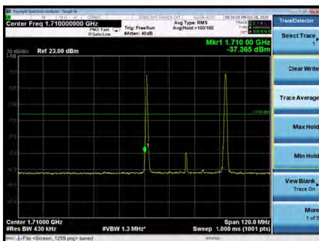
CA_66C 16QAM 20MHz+20MHz CH-Low, 1 RB
