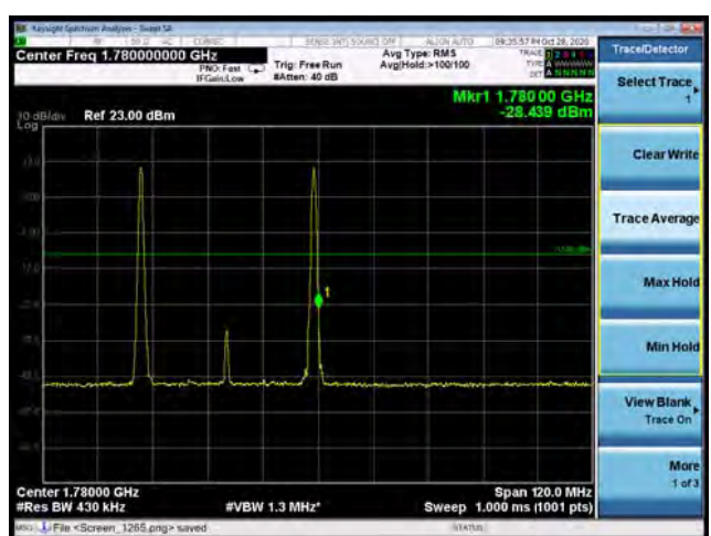
CA_66C 16QAM 20MHz+20MHz CH-High, 1 RB
