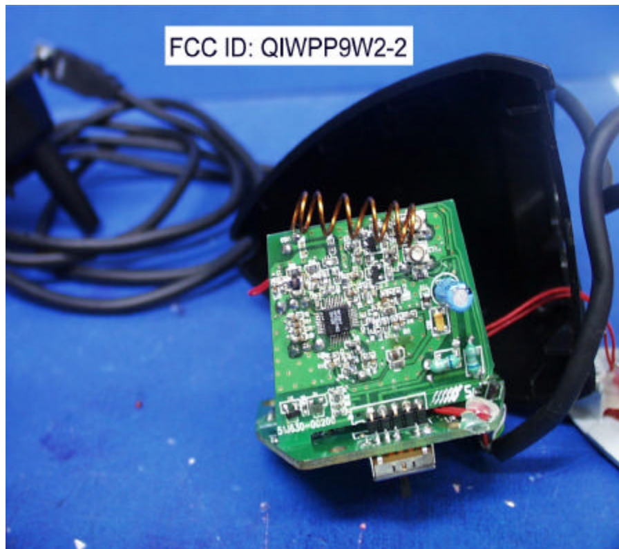
PCB Photo 3
