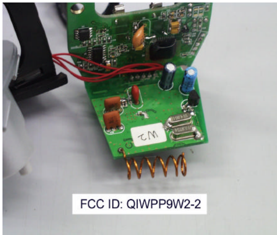
PCB Photo 2
