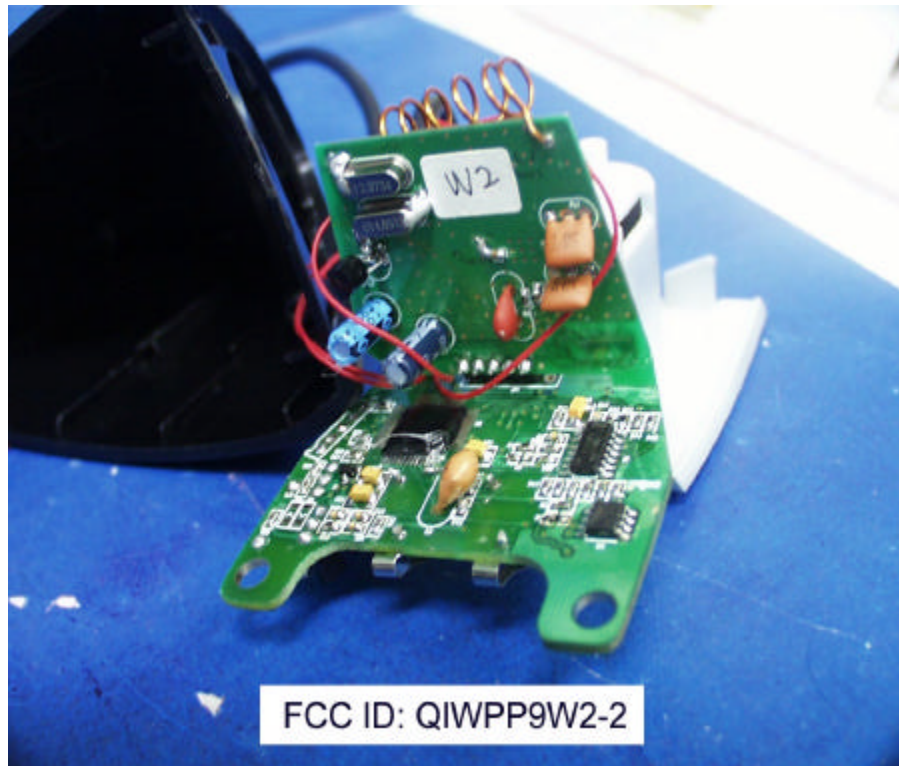
PCB Photo 5
