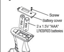
Diagram 1 BATTERY INSTALLATION
