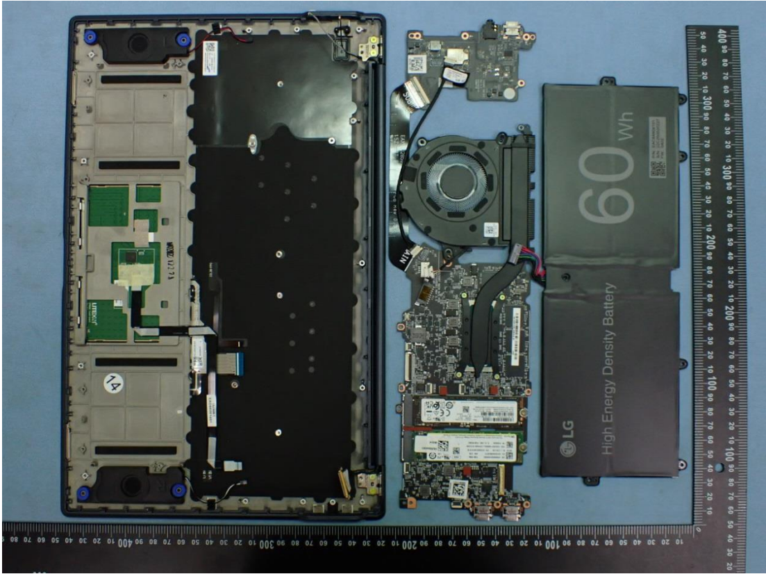
Figure 11 Internal View
