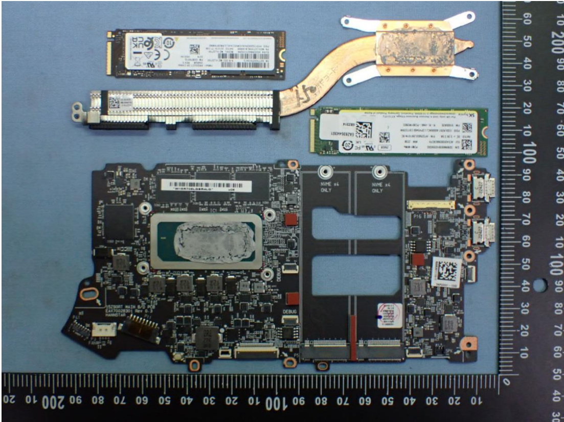
Figure 12 Internal View
