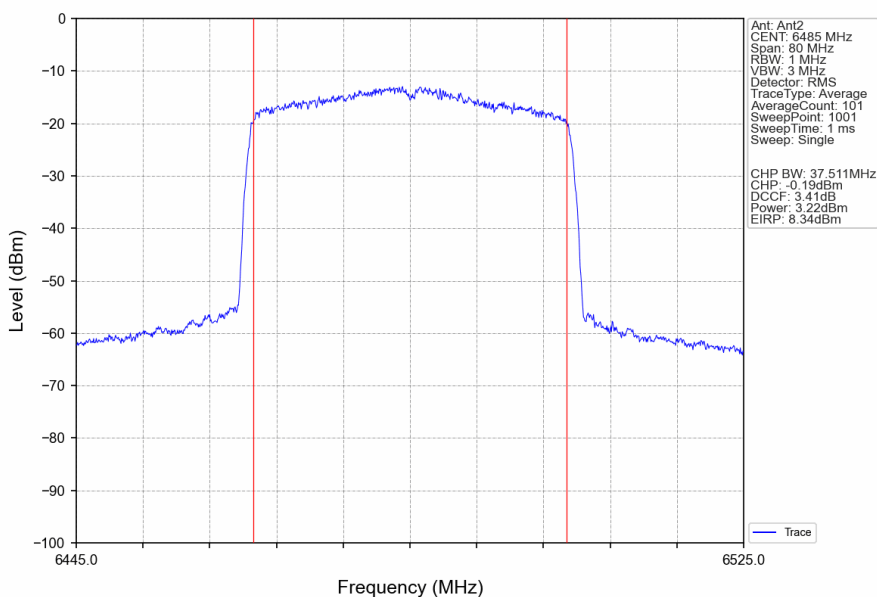
802.11ax(HEW40)_MCH_6485MHz_RU484_Left_Ant2_NTNV
