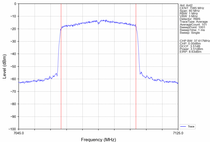
802.11ax(HEW40)_HCH_7085MHz_RU484_Left_Ant2_NTNV
