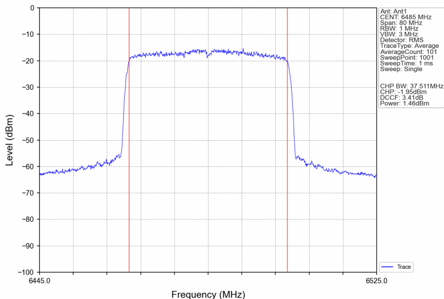
802.11ax(HEW40)_MCH_6485MHz_RU484_Left_Ant1_NTNV
