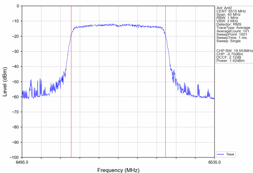
802.11ax(HEW20)_HCH_6515MHz_RU242_Left_Ant2_NTNV
