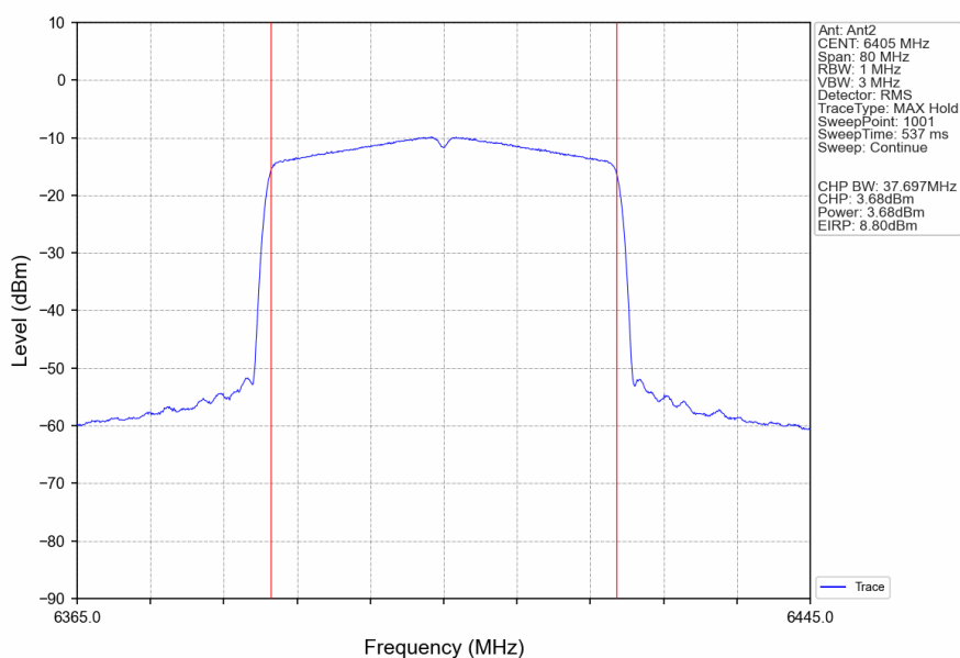
802.11ax(HEW40)_HCH_6405MHz_RU484_Left_Ant2_NTNV
