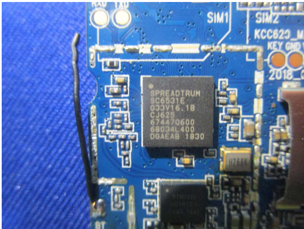
Main Chipset
