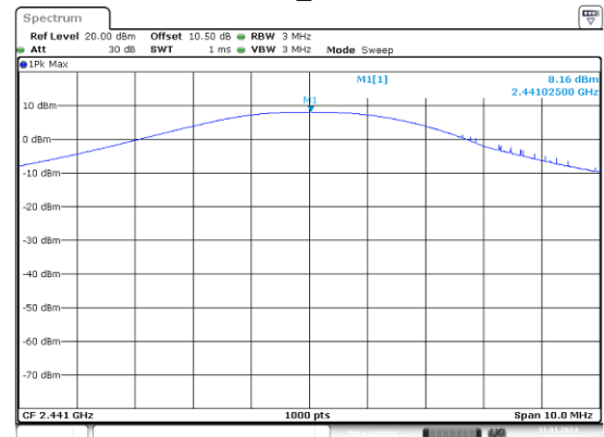
GFSK_Middle
