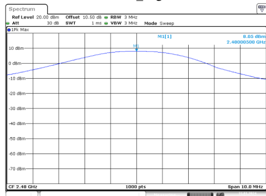
GFSK_High
