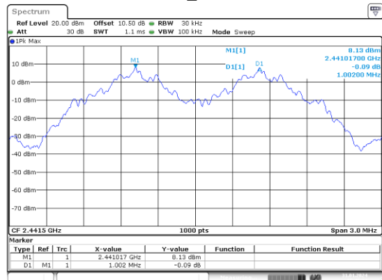
GFSK_Middle
