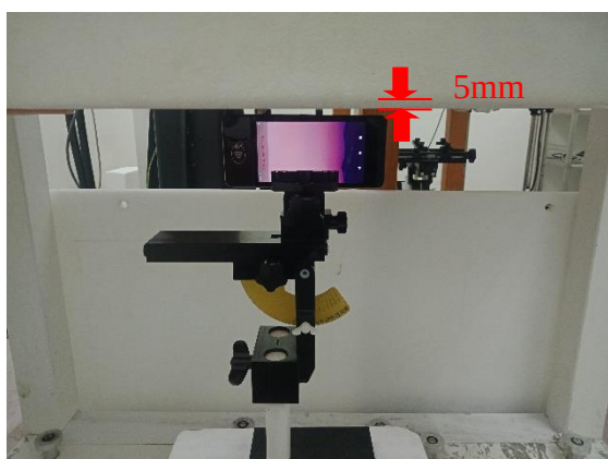
Photograph 11. Body, Right Edge, 5mm
