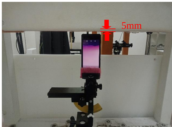
Photograph 7. Body, Bottom Edge, 5mm
