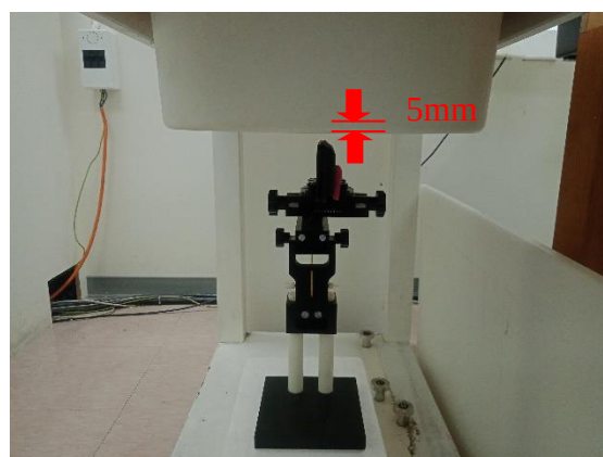
Photograph 12. Body, Right Edge, 5mm
