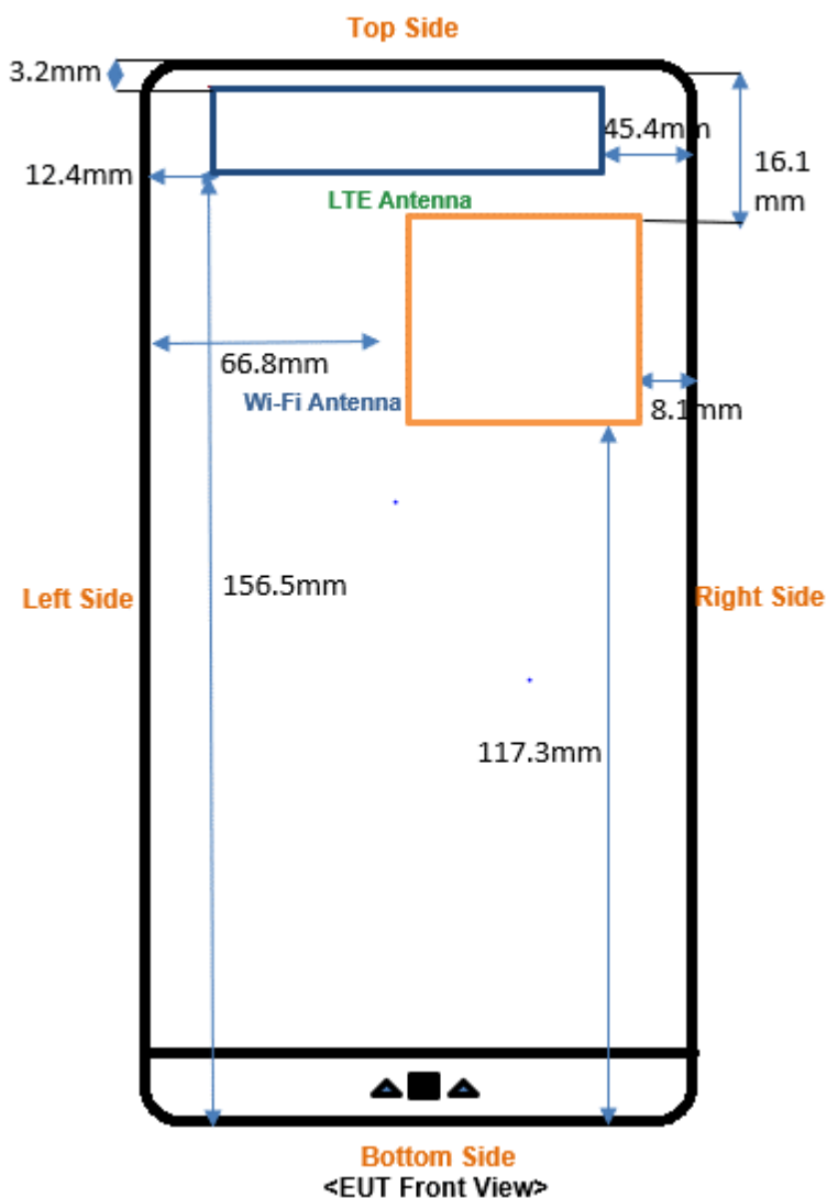
Photograph 15. Antenna position of EUT
