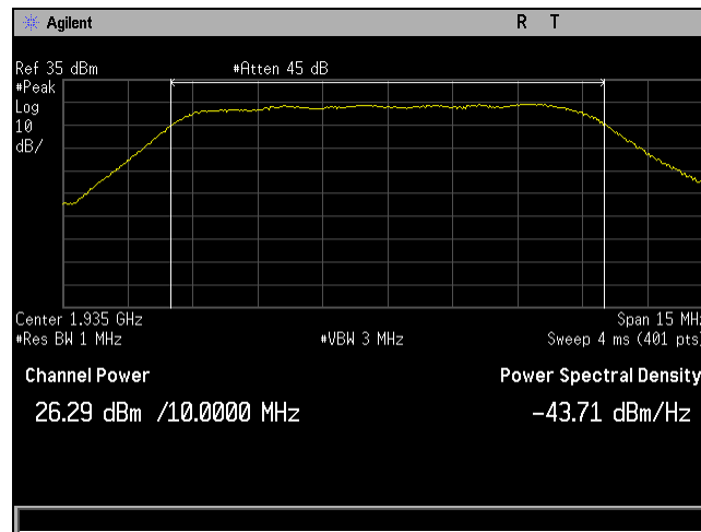
Plot 64. RF Output Power, QAM-16, 1935 MHz, Low Channel, Band 2, Port 2, Peak
