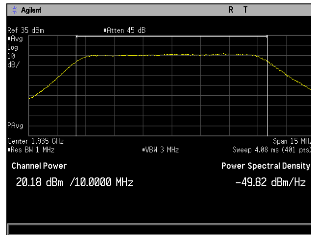
Plot 40. RF Output Power, QAM-64, 1935 MHz, Low Channel, Band 2, Port 1, Average
