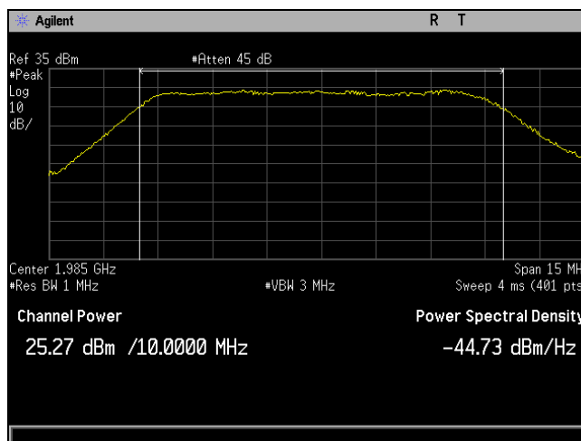
Plot 66. RF Output Power, QAM-16, 1985 MHz, High Channel, Band 2, Port 2, Peak
