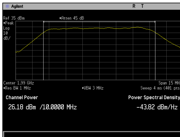
Plot 210. RF Output Power, QAM-16, 1990 MHz, High Channel, Band 25, Peak, Port 2, 10
