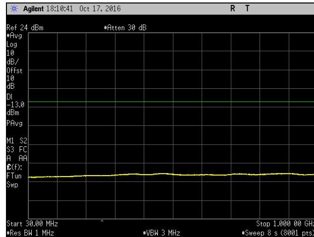
Plot 498. Conducted Spurious Emissions, Band 2, 30 MHz – 1 GHz, Low Channel, 20
