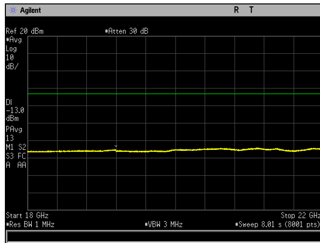
Plot 462. Conducted Spurious Emissions, Band 2, 18 GHz – 22 GHz, Low Channel, 10
