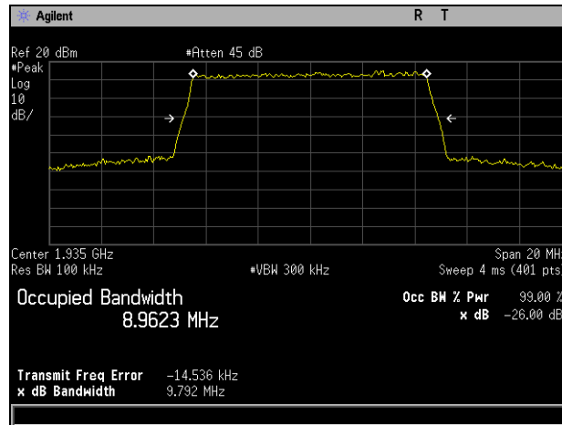
Plot 334. Occupied Bandwidth, QAM-16, Low Channel, Port 2, Band 2
