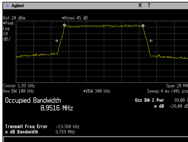
Plot 396. Occupied Bandwidth, QPSK, High Channel, Port 2, Band 25
