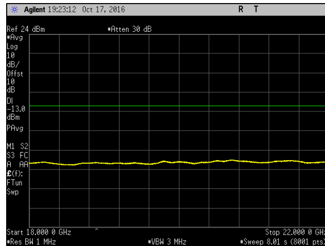
Plot 483. Conducted Spurious Emissions, Band 2, 18 GHz – 22 GHz, Low Channel, 15
