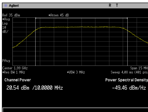
Plot 204. RF Output Power, QAM-64, 1990 MHz, High Channel, Band 25, Average, Port 2, 10
