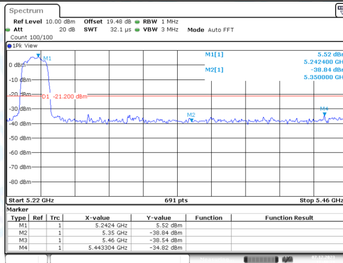
11N20SISO_Ant1_High_5240_Peak
