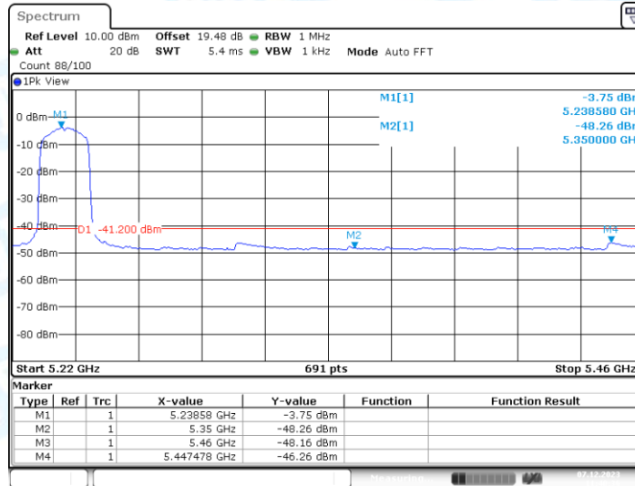
11N20SISO_Ant1_High_5240_AV
