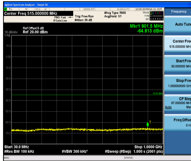
Band7_15MHz_16QAM_21375_1RB#0_30~1000_30~1000
