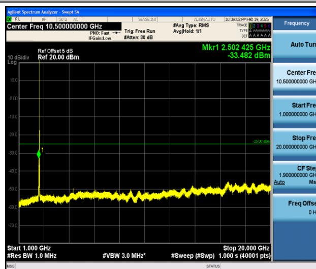
Band7_15MHz_QPSK_21375_1RB#0_1000~20000_1000~20000
