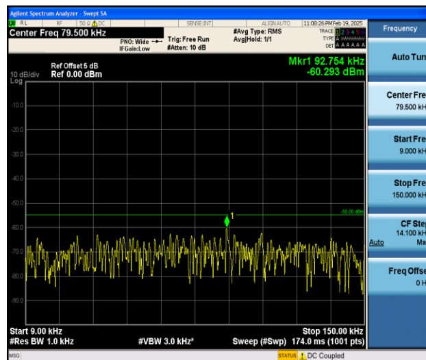
Band7_20MHz_QPSK_21100_1RB#0_0.009~0.15_0.009~0.15
