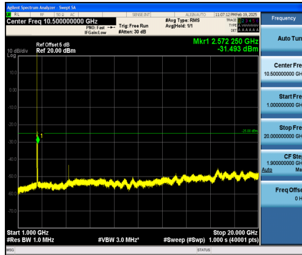
Band7_20MHz_QPSK_20850_1RB#0_1000~20000_1000~20000
