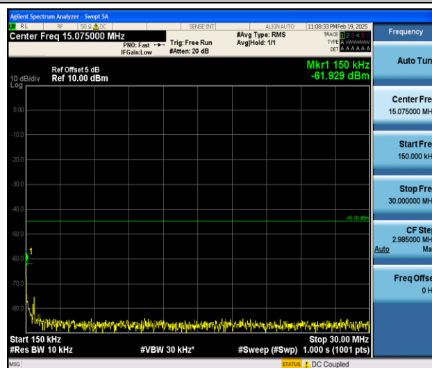
Band7_20MHz_QPSK_21100_1RB#0_0.15~30_0.15~30
