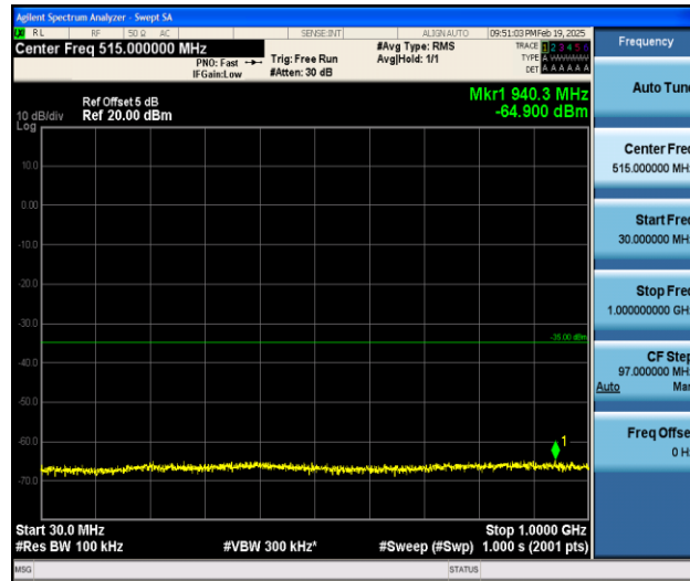
Band7_10MHz_16QAM_21400_1RB#0_30~1000_30~1000
