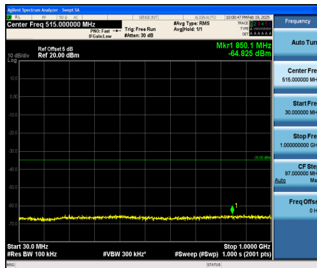
Band7_15MHz_QPSK_21375_1RB#0_30~1000_30~1000
