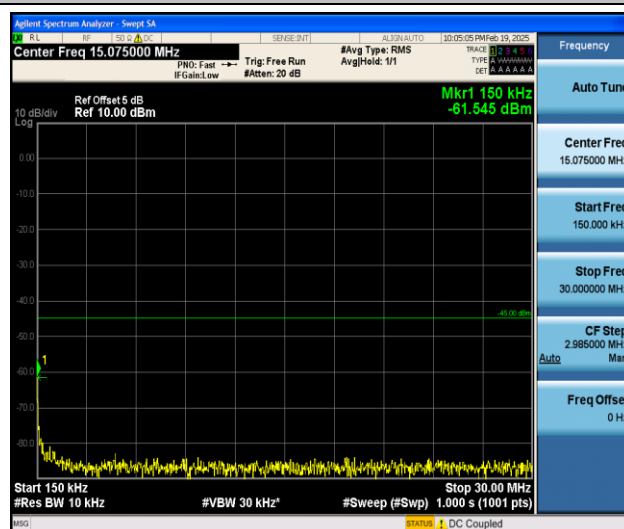
Band7_15MHz_QPSK_21100_1RB#0_0.15~30_0.15~30
