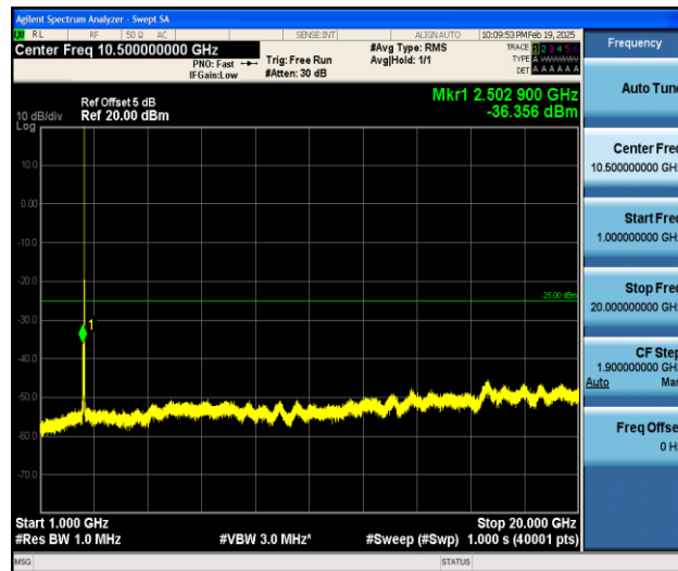
Band7_15MHz_16QAM_21375_1RB#0_1000~20000_1000~20000
