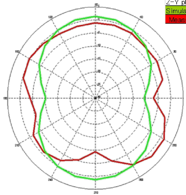
Z-Y Plane
