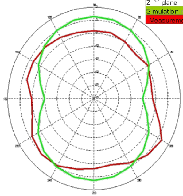
Z-Y Plane
