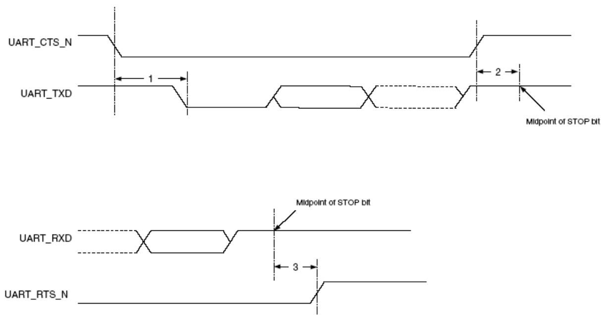
Figure 12. UART Timing
