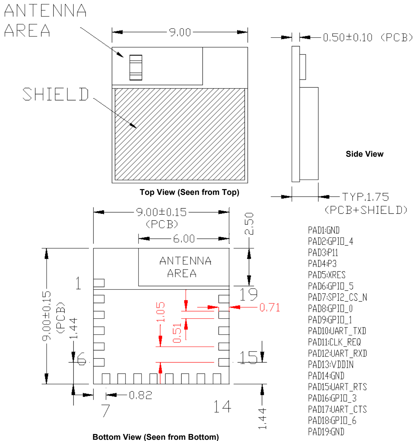
Figure 2. Module Mechanical Drawing
