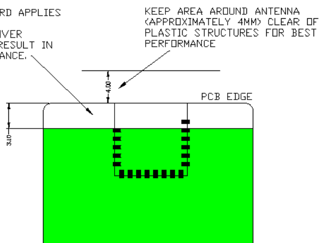
Figure 4. Recommended Host PCB Keep Out Area Around the CYBT-353027-02 Antenna
