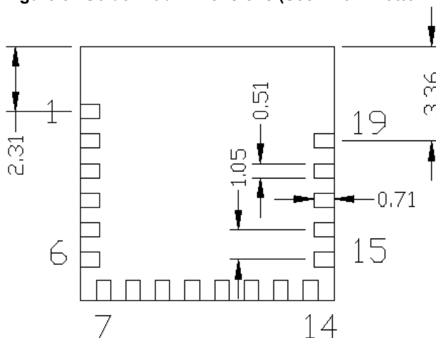
Figure 3. Solder Pad Dimensions (Seen from Bottom)
