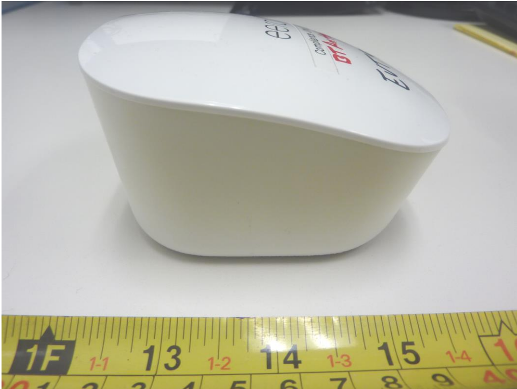
Figure 5 - External Photo of EUT- Left View
