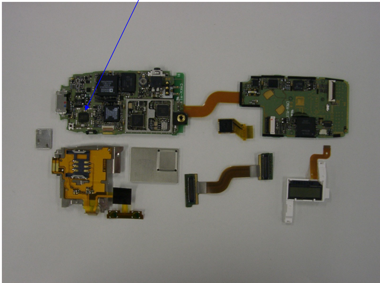
Bluetooth Chip
