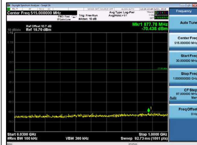
CUE-802.11n-20-5500M-chain2(30MHz-1GHz)
