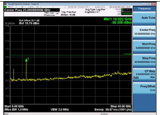
CUE-802.11n-40-5270M-chain4(6GHz-40GHz)
