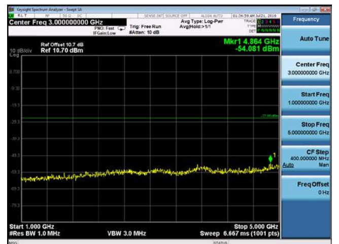
CUE-802.11ac-80-5290M-chain 3(1GHz-5GHz)
