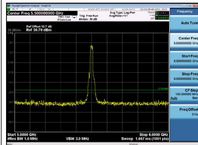
CUE-802.11n-20-5500M-chain3(5GHz-6GHz)
