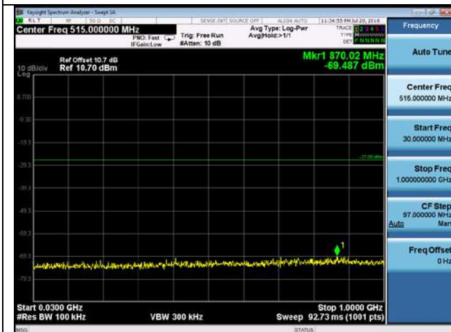
CUE-802.11a-5700M-chain 1(30MHz-1GHz)
