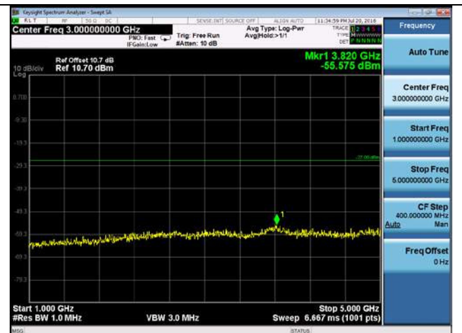
CUE-802.11a-5700M-chain 1(1GHz-5GHz)
