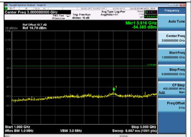
CUE-802.11a-5500M -chain3(1GHz-5GHz)
