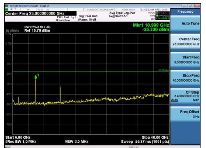
CUE-802.11a-5500M-chain3(6GHz-40GHz)
