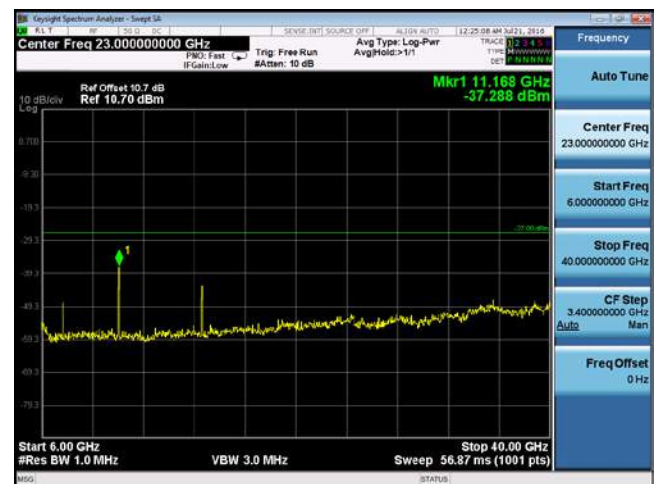
CUE-802.11n-20-5580M-chain2(6GHz-40GHz)
