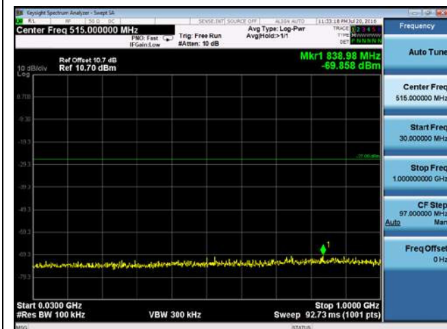
CUE-802.11a-5580M-chain1(30MHz-1GHz)
