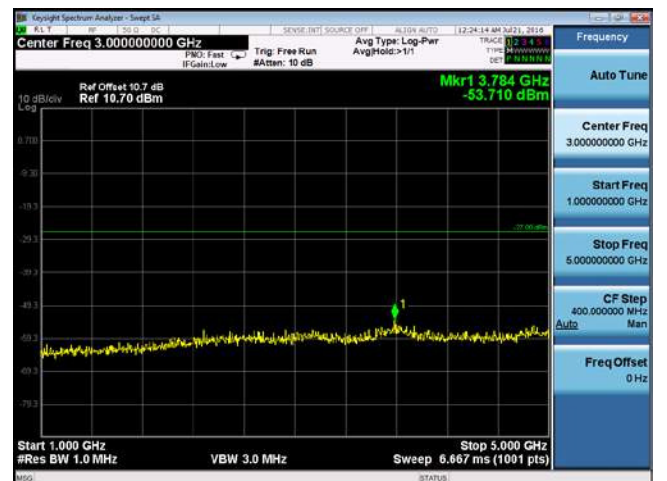
CUE-802.11n-20-5500M-chain2(1GHz-5GHz)
