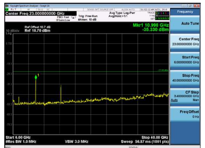
CUE-802.11n-20-5500M-chain3(6GHz-40GHz)
