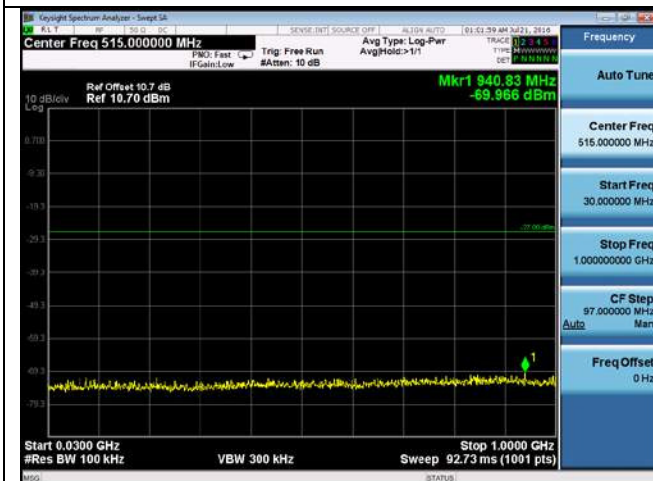
CUE-802.11a-5500M -chain3(30MHz-1GHz)
