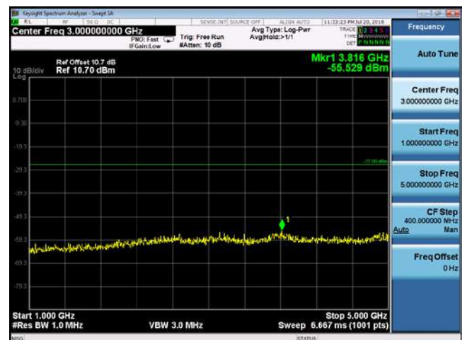
CUE-802.11a-5580M-chain1(1GHz-5GHz)
