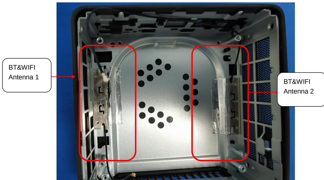
INTERNAL VIEW OF EUT (FIGURE 8)
