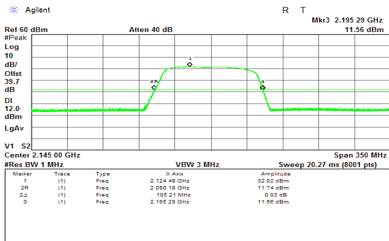
Plot 7.4.1 Out-of-band rejection test result
