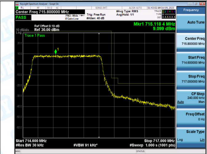
Band12_1.4MHz_16QAM_23173_6RB#0
