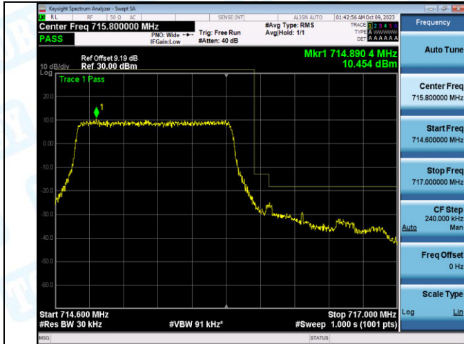
Band12_1.4MHz_QPSK_23173_6RB#0
