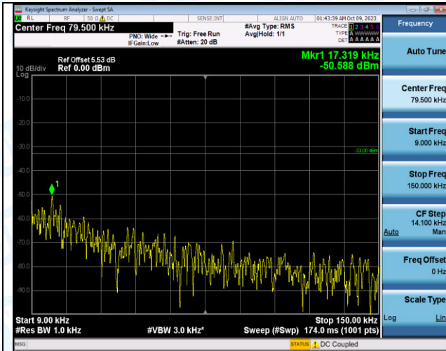
Band12_1.4MHz_QPSK_23017_1RB#0_0.009~0.15_0.00 9~0.15
