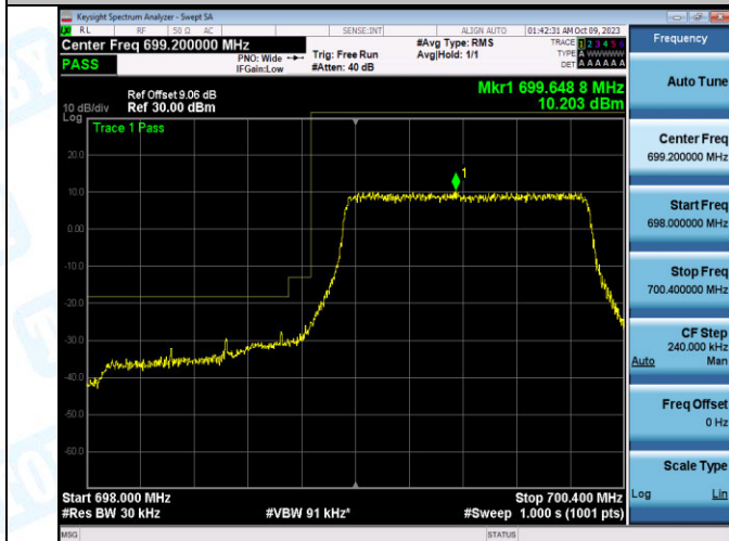
Band12_1.4MHz_QPSK_23017_6RB#0
