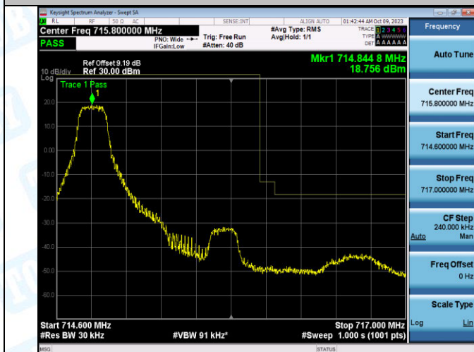
Band12_1.4MHz_QPSK_23173_1RB#0
