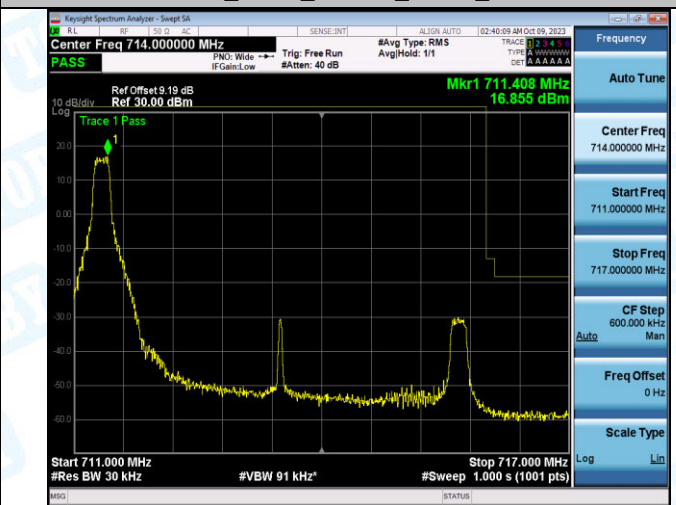
Band12_5MHz_16QAM_23155_1RB#0
