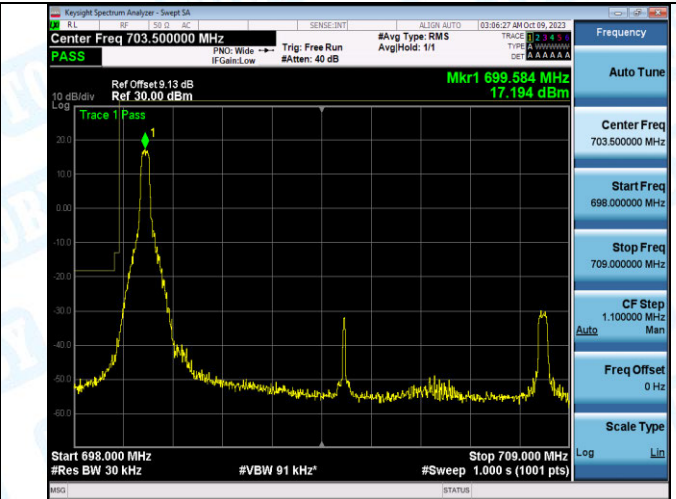
Band12_10MHz_16QAM_23060_1RB#0
