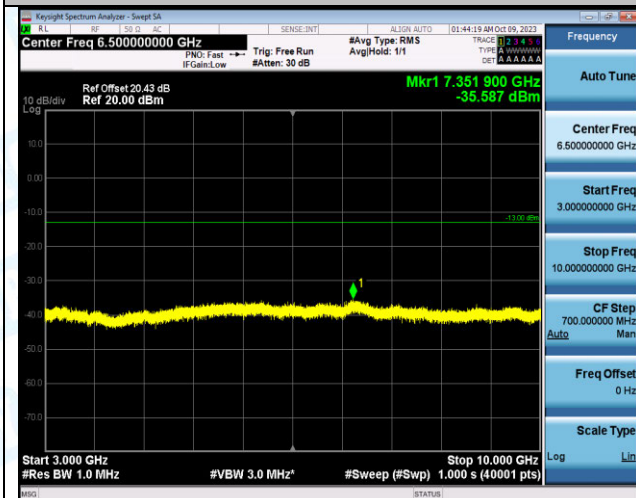
Band12_1.4MHz_QPSK_23017_1RB#0_3000~10000_30 00~10000
