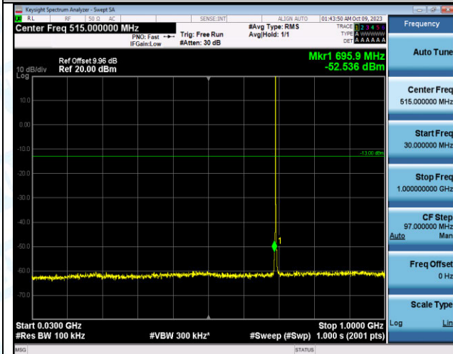
Band12_1.4MHz_QPSK_23017_1RB#0_30~1000_30~10 00
