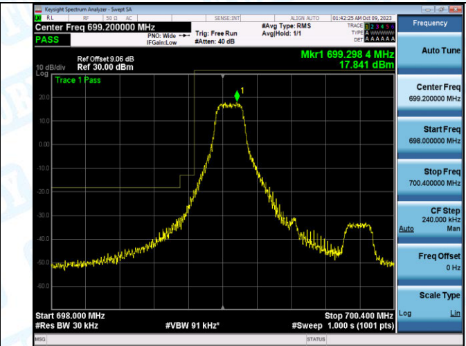
Band12_1.4MHz_16QAM_23017_1RB#0
