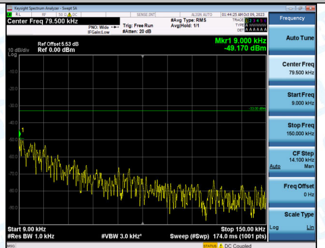
Band12_1.4MHz_16QAM_23017_1RB#0_0.009~0.15_0.0 09~0.15
