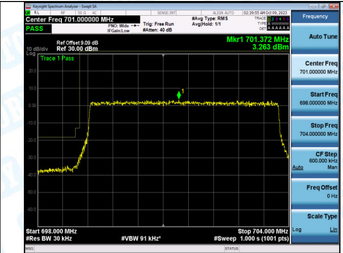
Band12_5MHz_16QAM_23035_25RB#0
