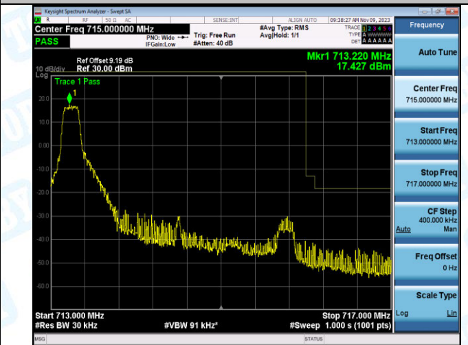
Band12_3MHz_16QAM_23165_1RB#0
