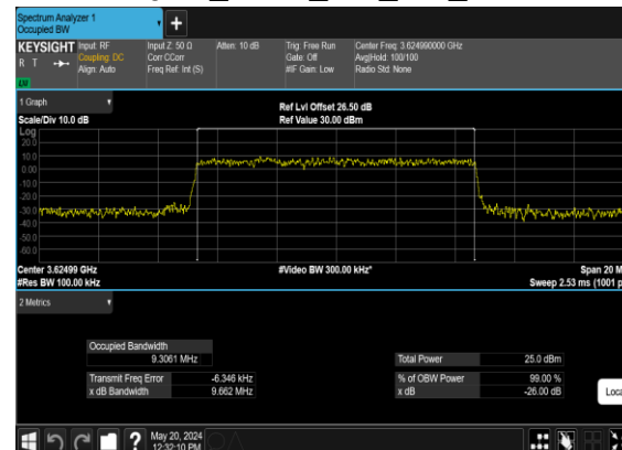
N48(10M)_CP-OFDM_16 QAM_Outer_Full_Mid_CH
