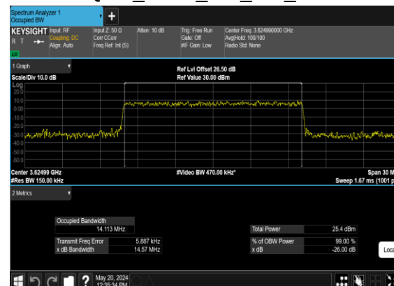
N48(15M)_CP-OFDM_16 QAM_Outer_Full_Mid_CH
