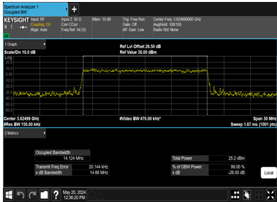
N48(15M)_CP-OFDM_64 QAM_Outer_Full_Mid_CH
