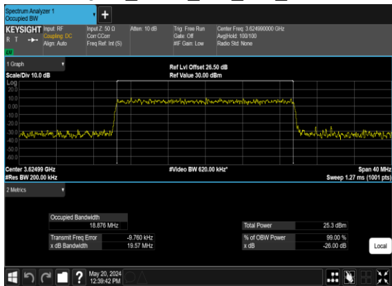
N48(20M)_CP-OFDM_64 QAM_Outer_Full_Mid_CH
