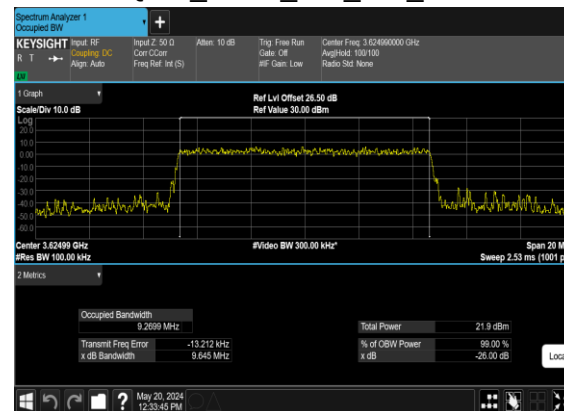
N48(10M)_CP-OFDM_256 QAM_Outer_Full_Mid_CH
