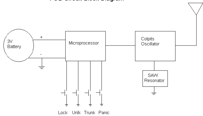
FOB Circuit Block Diagram
