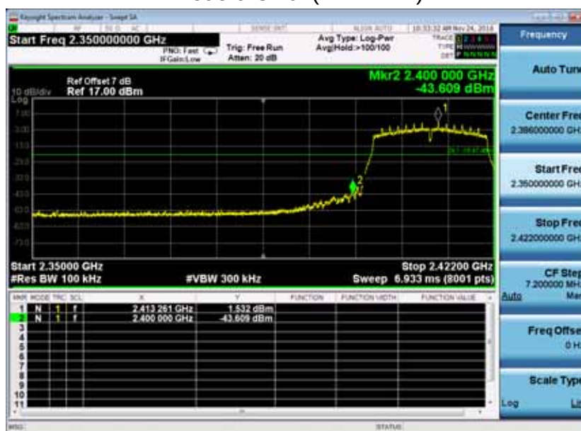
Mode 9 CH01(2412MHz)
