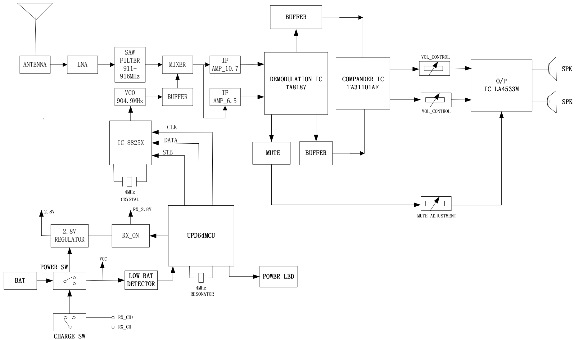
Block Diagram
