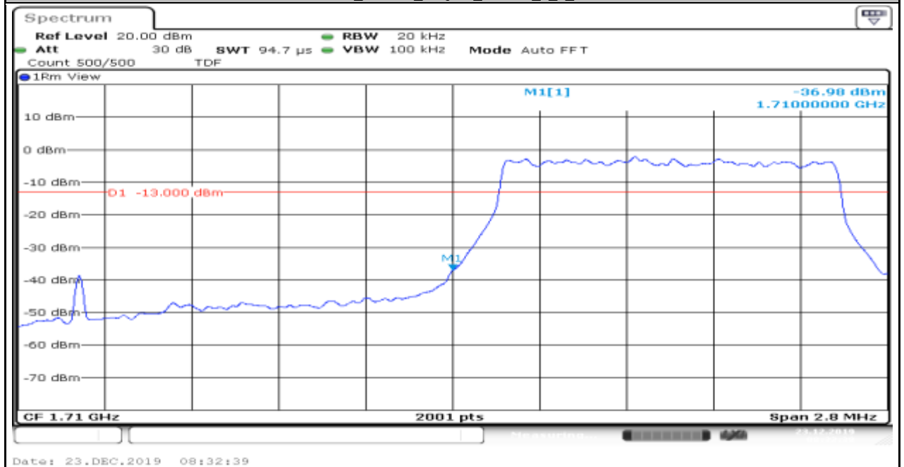
Band66_1.4MHz_16QAM_131979_1_0_Low
