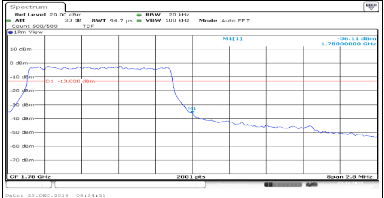
Band66_1.4MHz_QPSK_132665_1_5_Low
