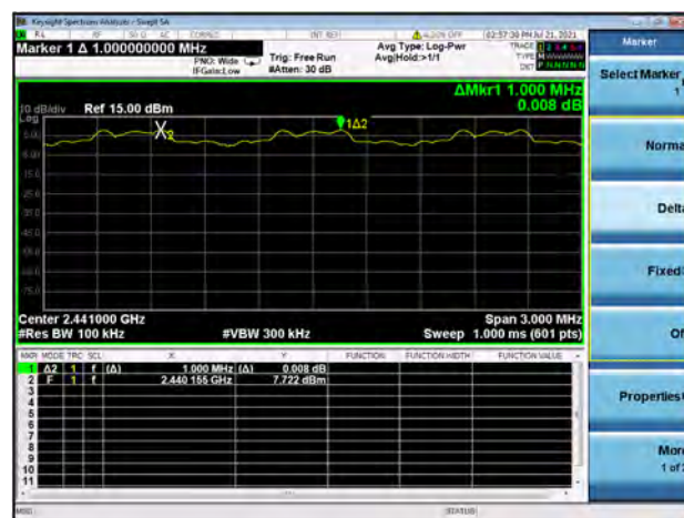
8-DPSK
