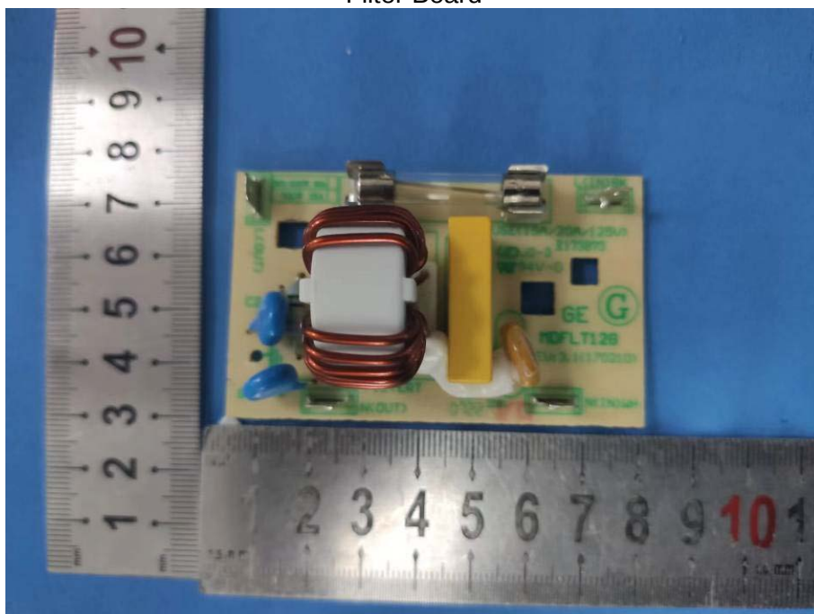
Filter Board
