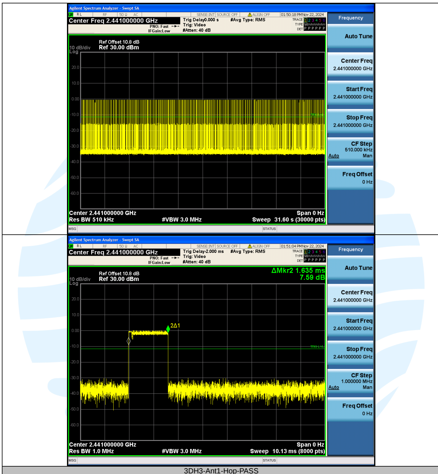
3DH3-Ant1-Hop-PASS
