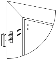
Figure 6: Magnet screw installation
