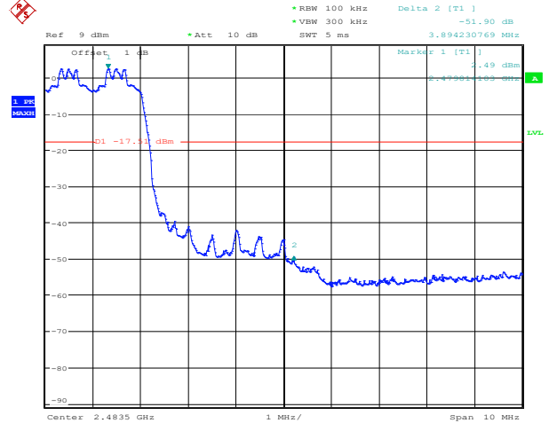
GFSK / Hopping
