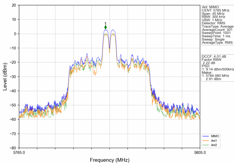
802.11ax(HEW20)_MCH_5785MHz_RU26_Mid_MIMO_NTNV
