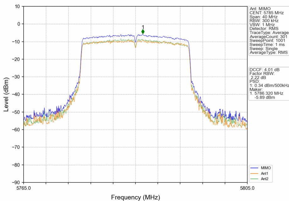
802.11ax(HEW20)_MCH_5785MHz_RU242_Left_MIMO_NTNV
