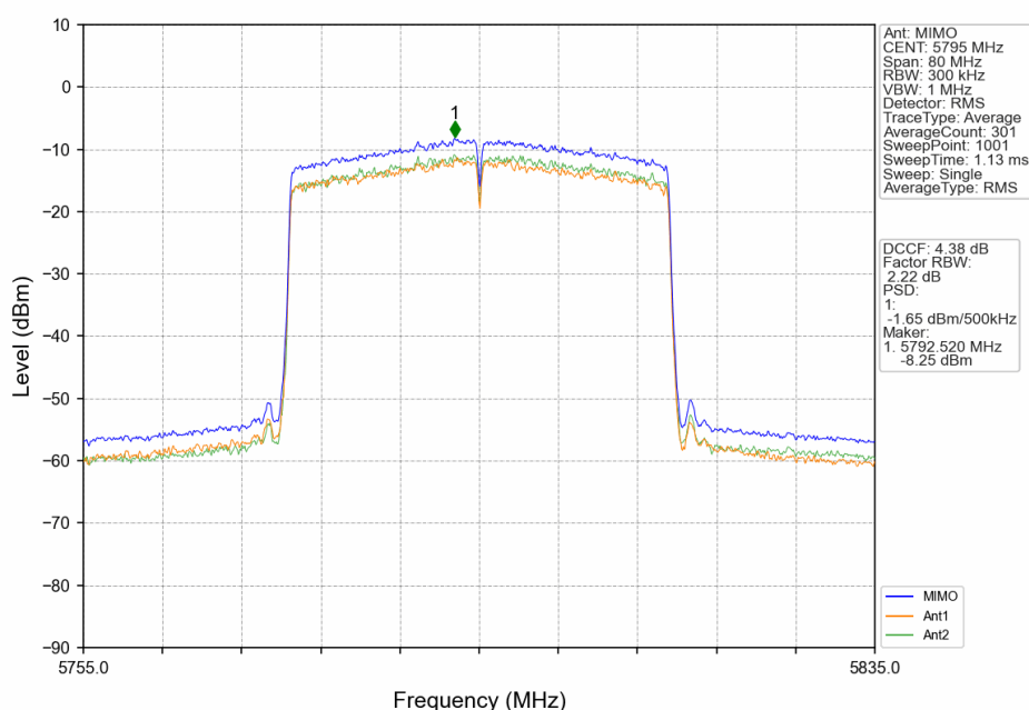
802.11ax(HEW40)_HCH_5795MHz_RU484_Left_MIMO_NTNV
