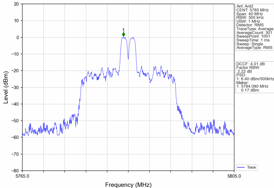
802.11ax(HEW20)_MCH_5785MHz_RU26_Mid_MIMO_NTNV
