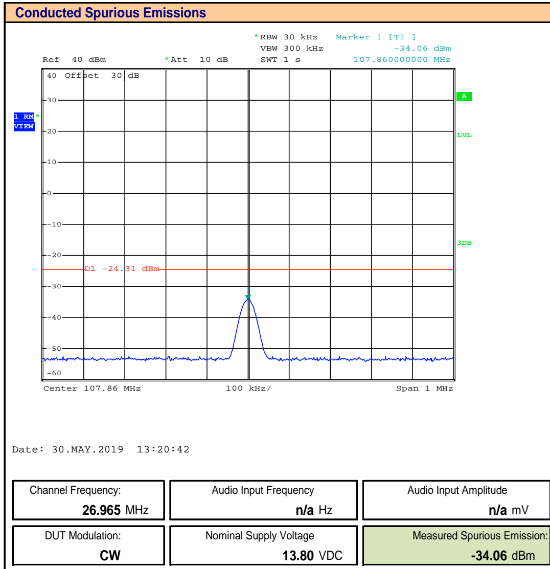
Plot 10.6 – Conducted Out of Band Emissions, Channel 1, 4th Harmonic
