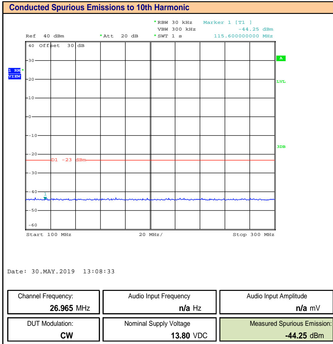
Plot 10.3 – Conducted Out of Band Emissions, 100MHz – 300MHz, Channel 1
