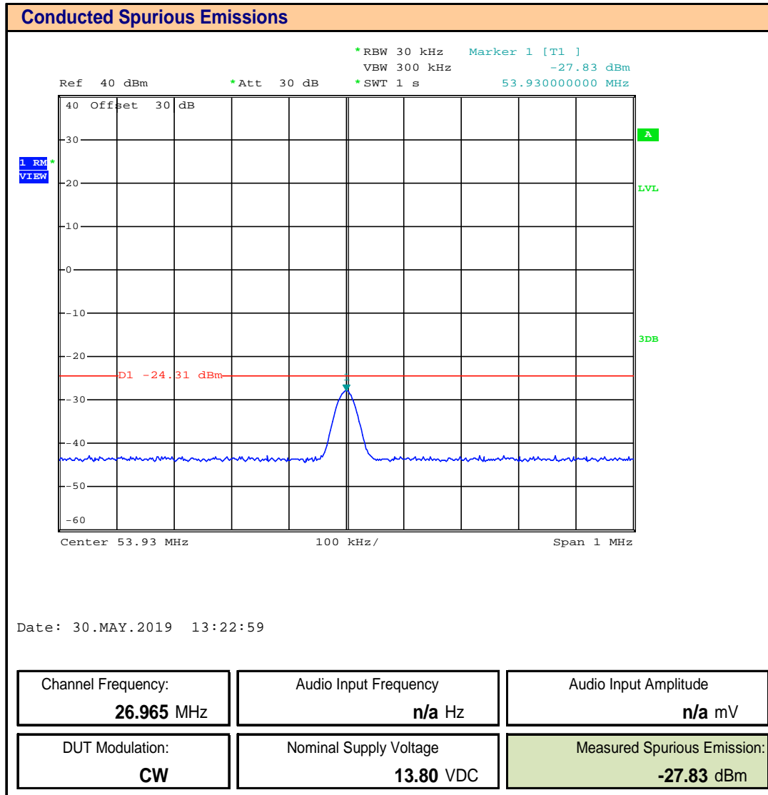
Plot 10.4 – Conducted Out of Band Emissions, Channel 1, 2 nd Harmonic
