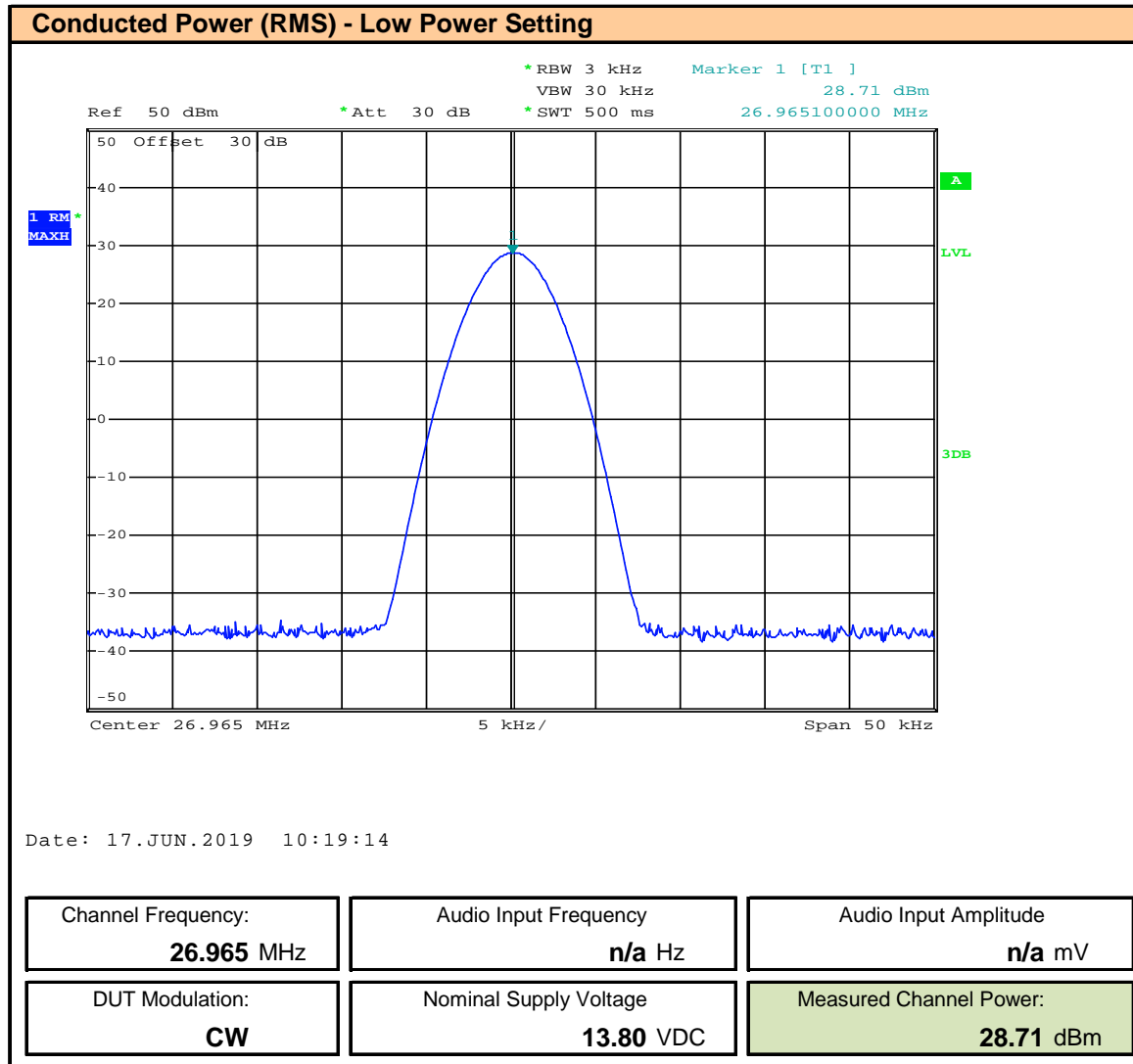
Plot 7.4 – Conducted Output Power – Channel 1 – Low Power
