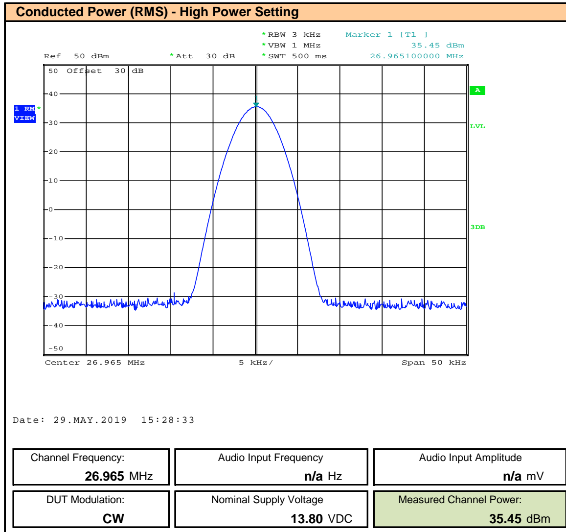
Plot 7.1 – Conducted Output Power – Channel 1 – High Power
