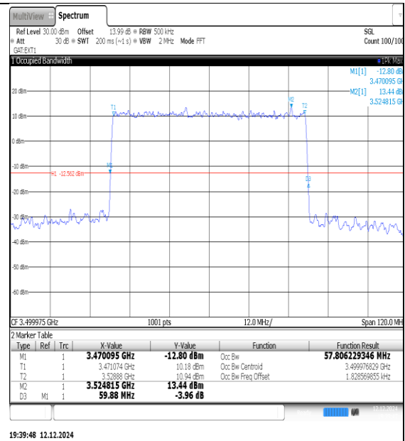
NTNV-N77-3450-3550-PC3-30-70-M-DFT-16QAM-Outer_Full-Ant1-PASS
