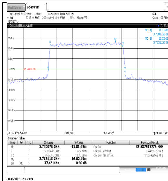
NTNV-N78-3700-3800-PC3-30-50-M-DFT-QPSK-Outer_Full-Ant1-PASS
