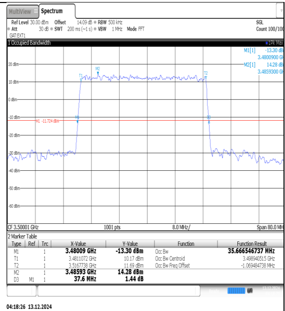
NTN-N78-3450-3550-PC3-30-50-M-DFT-16QAM-Outet_Full-Ant1-PASS
