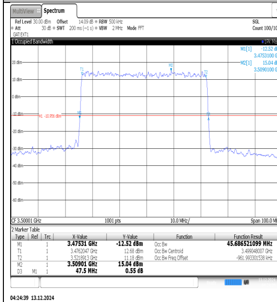
NTN-N78-3450-3550-PC3-30-60-M-DFT-QPSK-Outet_Full-Ant1-PASS
