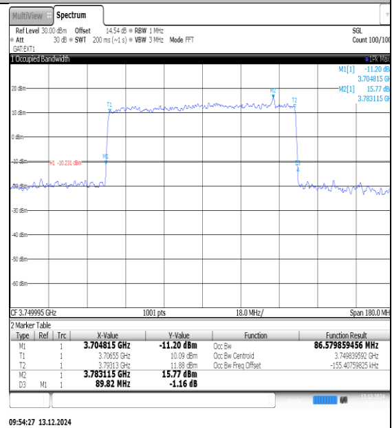
NTNV-N78-3700-3800-PC3-30-100-M-DFT-16QAM-Outer_Full-Ant1-PASS
