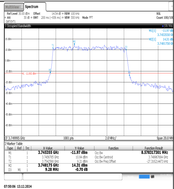
NTNV-N78-3700-3800-PC3-30-15-M-DFT-16QAM-Outet_Full-Ant1-PASS
