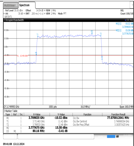
NTNV-N78-3700-3800-PC3-30-90-M-DFT-16QAM-Outer_Full-Ant1-PASS
