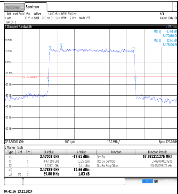
NTNV-N78-3450-3550-PC3-30-70-M-DFT-16QAM-Outer_Full-Ant1-PASS
