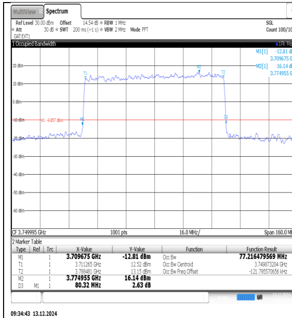
NTNV-N78-3700-3800-PC3-30-90-M-DFT-QPSK-Outer_Full-Ant1-PASS
