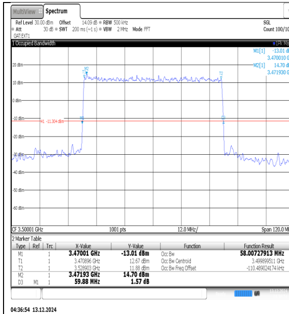
NTNV-N78-3450-3550-PC3-30-70-M-DFT-QPSK-Outer_Full-Ant1-PASS
