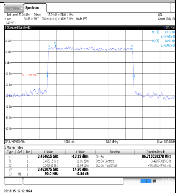
NTNV-N77-3450-3550-PC3-30-100-M-DFT-16QAM-Outer_Full-Ant1-PASS
