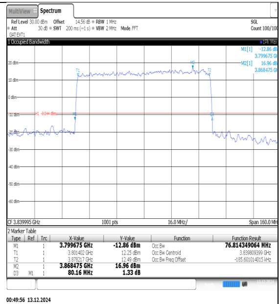
NTNV-N77-3700-3980-PC3-30-90-M-DFT-16QAM-Outer_Full-Ant1-PASS
