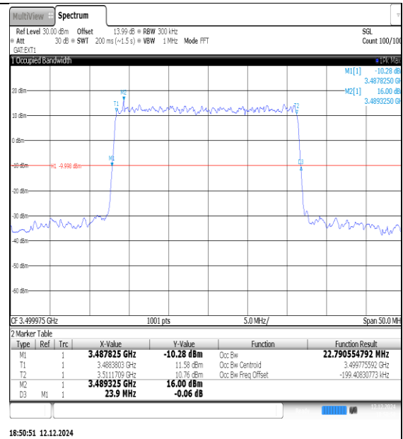
NTNV-N77-3450-3550-PC3-30-30-M-DFT-16QAM-Outet_Full-Ant1-PASS
