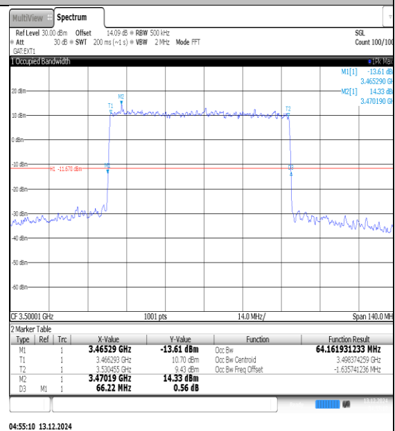
NTNV-N78-3450-3550-PC3-30-80-M-DFT-16QAM-Outer_Full-Ant1-PASS
