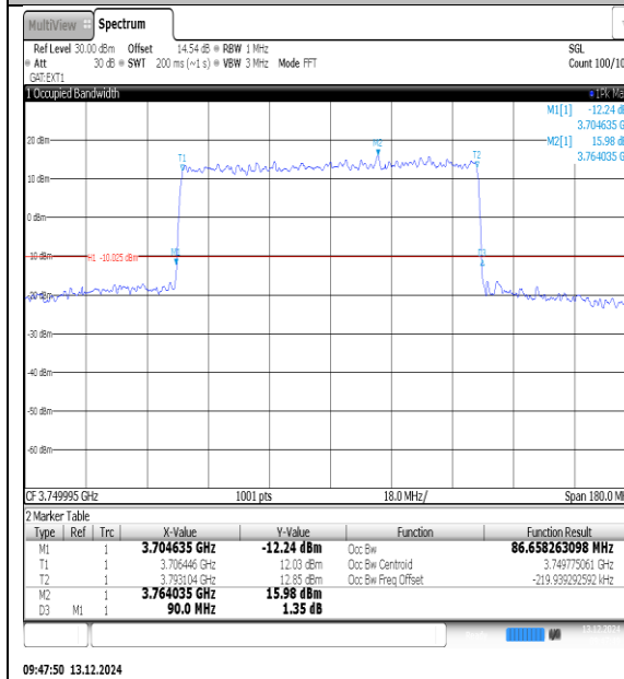
NTNV-N78-3700-3800-PC3-30-100-M-DFT-QPSK-Outer_Full-Ant1-PASS
