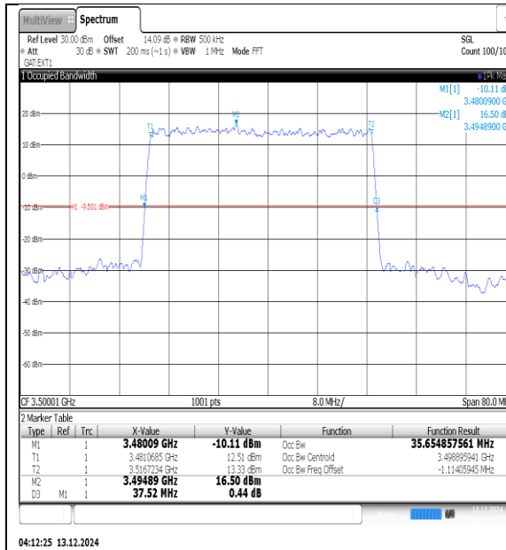
NTN-N78-3450-3550-PC3-30-50-M-DFT-QPSK-Outet_Full-Ant1-PASS
