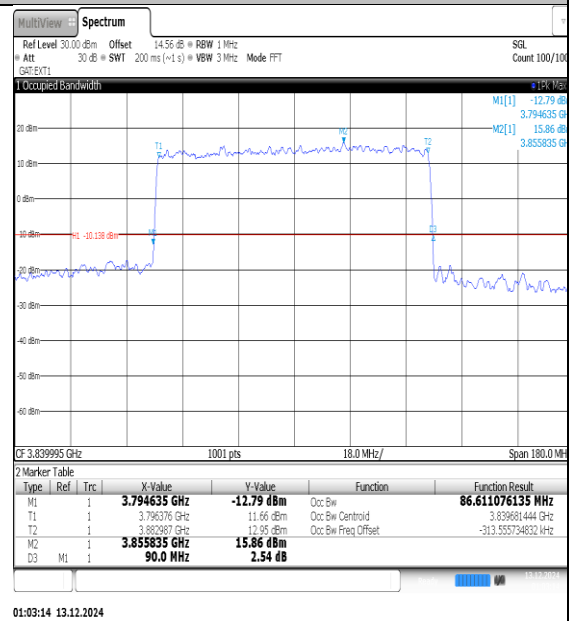
NTNV-N77-3700-3980-PC3-30-100-M-DFT-16QAM-Outer_Full-Ant1-PASS
