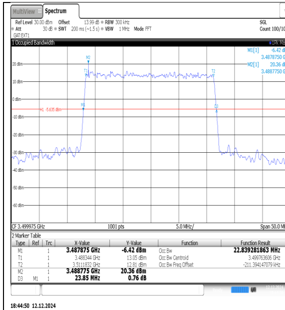
NTNV-N77-3450-3550-PC3-30-30-M-DFT-QPSK-Outet_Full-Ant1-PASS
