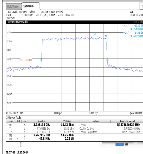
NTNV-N78-3700-3800-PC3-30-60-M-DFT-QPSK-Outer_Full-Ant1-PASS
