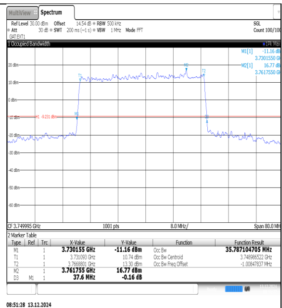
NTNV-N78-3700-3800-PC3-30-50-M-DFT-16QAM- Outer_Full-Ant1-PASS
