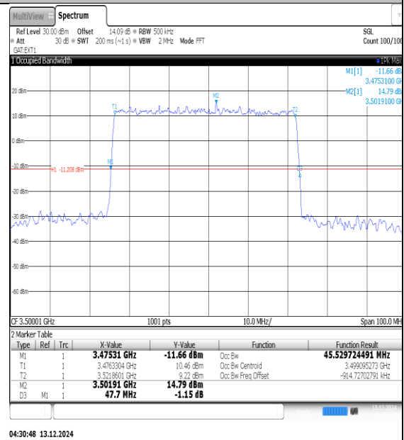
NTN-N78-3450-3550-PC3-30-60-M-DFT-16QAM-Outet_Full-Ant1-PASS
