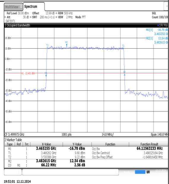
NTNV-N77-3450-3550-PC3-30-80-M-DFT-16QAM-Outer_Full-Ant1-PASS
