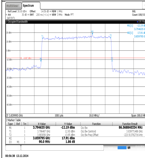
NTNV-N77-3700-3980-PC3-30-100-M-DFT-QPSK-Outer_Full-Ant1-PASS
