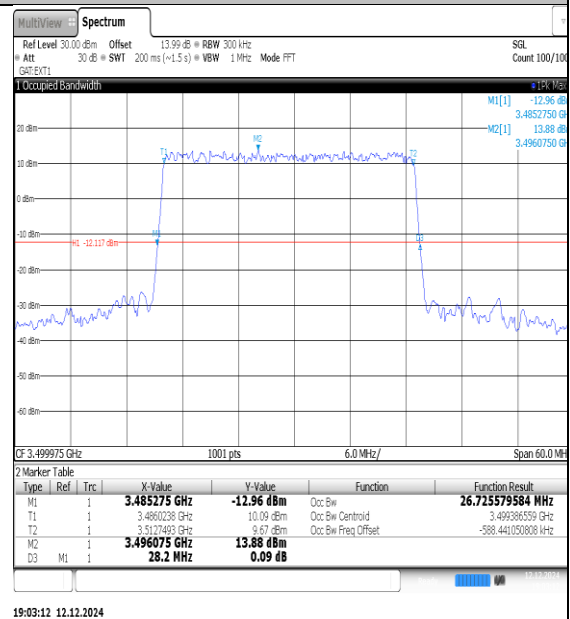
NTNV-N77-3450-3550-PC3-30-40-M-DFT-16QAM-Outet_Full-Ant1-PASS
