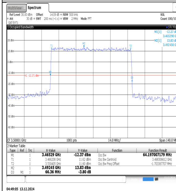
NTNV-N78-3450-3550-PC3-30-80-M-DFT-QPSK-Outer_Full-Ant1-PASS
