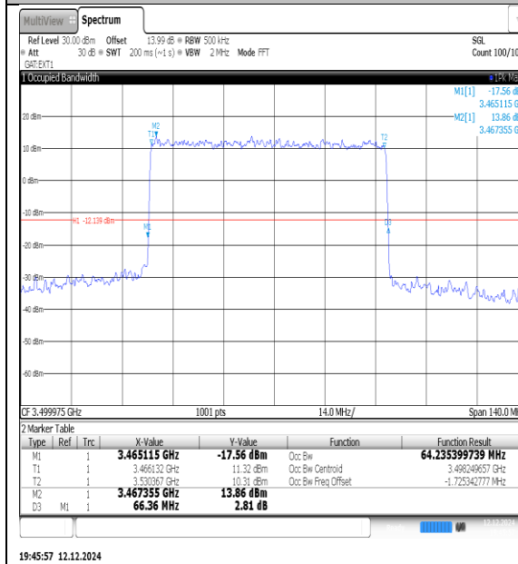
NTNV-N77-3450-3550-PC3-30-80-M-DFT-QPSK-Outer_Full-Ant1-PASS
