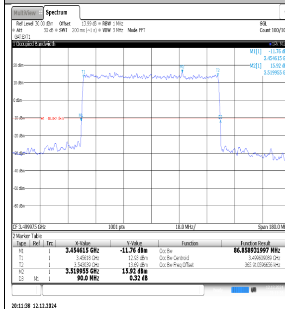
NTNV-N77-3450-3550-PC3-30-100-M-DFT-QPSK-Outer_Full-Ant1-PASS
