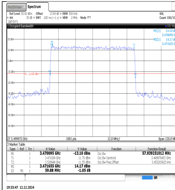
NTNV-N77-3450-3550-PC3-30-70-M-DFT-QPSK-Outer_Full-Ant1-PASS
