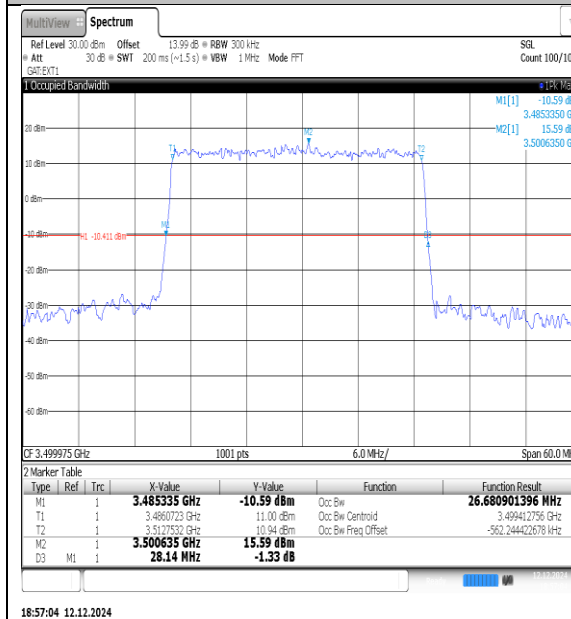
NTNV-N77-3450-3550-PC3-30-40-M-DFT-QPSK-Outet_Full-Ant1-PASS
