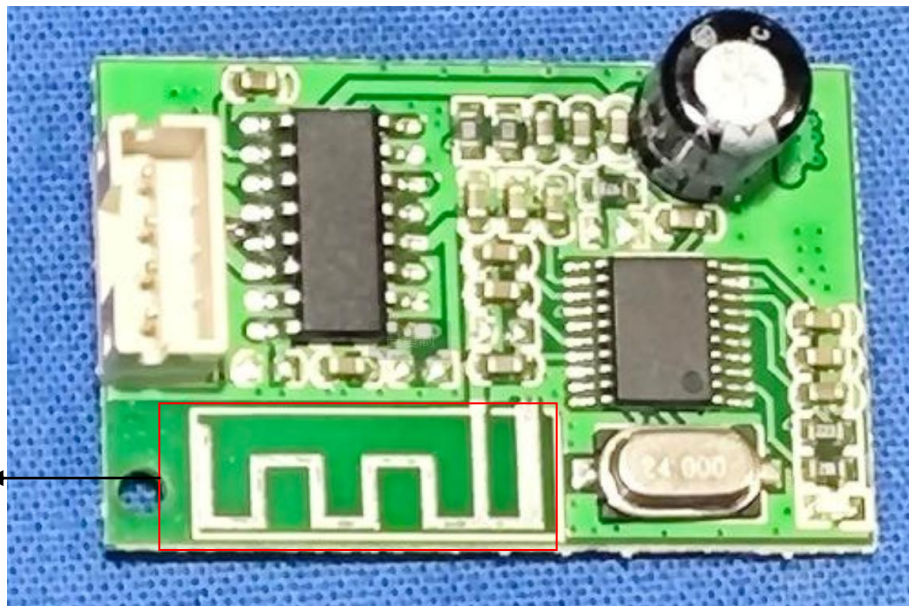
2402-2480MHz Antenna
