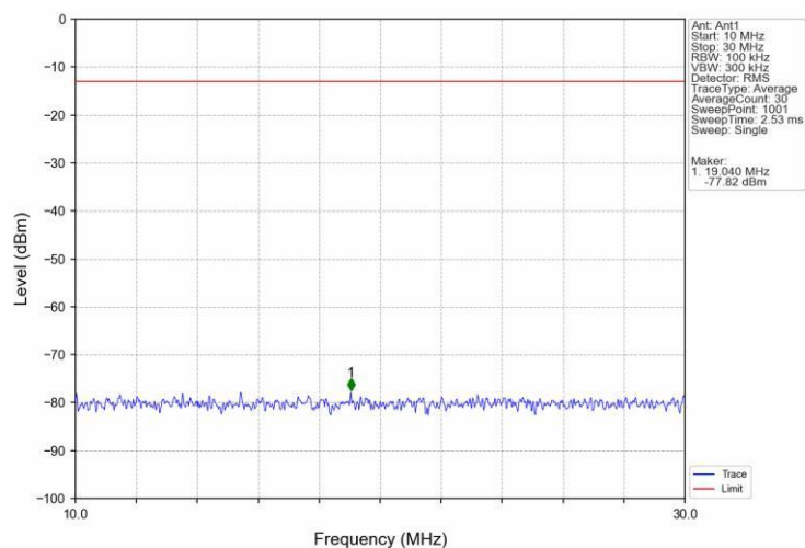
Band25_10MHz_16QAM_MCH_1882.5MHz_RB_1_0_NTNV
