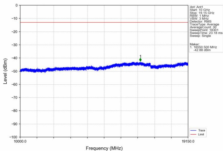
Band25_15MHz_QPSK_LCH_1857.5MHz_RB_1_0_NTNV
