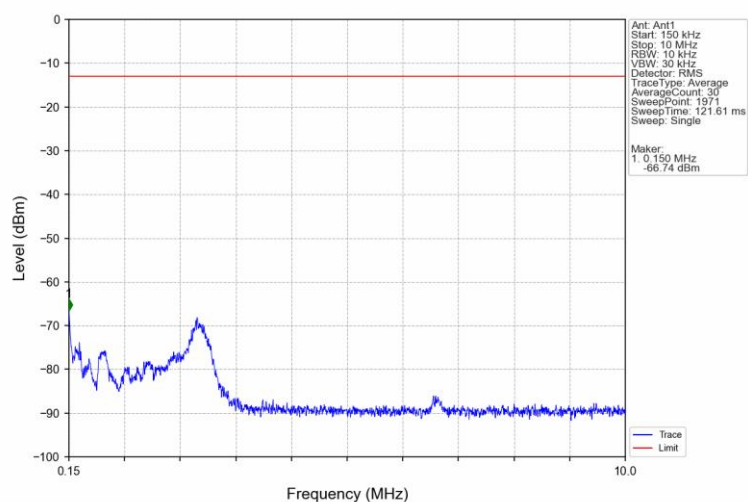
Band25_15MHz_QPSK_MCH_1882.5MHz_RB_1_0_NTNV
