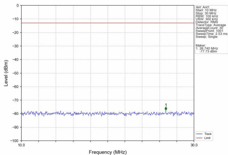
Band25_10MHz_QPSK_MCH_1882.5MHz_RB_1_0_NTNV
