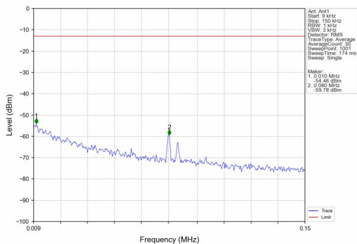
Band25_15MHz_16QAM_HCH_1907.5MHz_RB_1_0_NTNV
