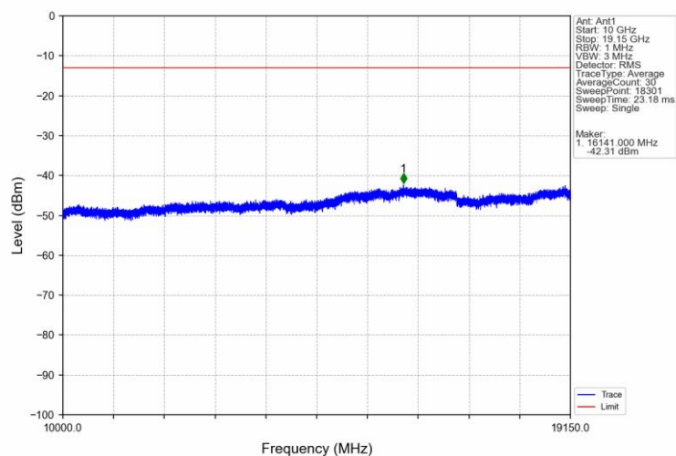
Band25_15MHz_16QAM_HCH_1907.5MHz_RB_1_0_NTNV
