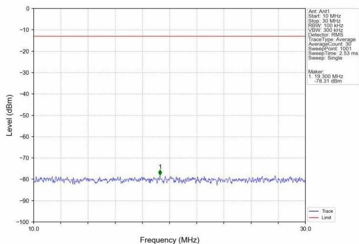
Band25_15MHz_16QAM_MCH_1882.5MHz_RB_1_0_NTNV
