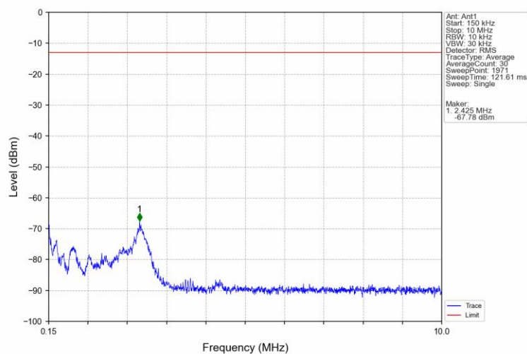
Band25_10MHz_16QAM_MCH_1882.5MHz_RB_1_0_NTNV
