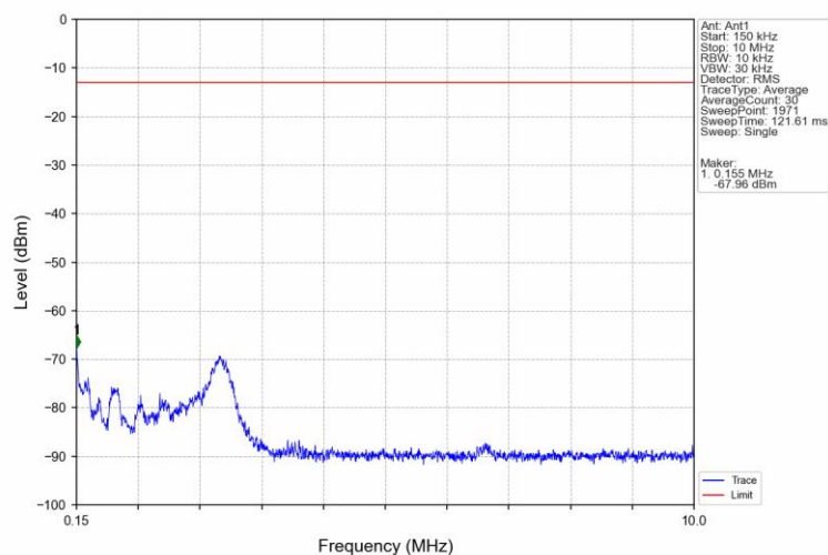
Band25_15MHz_16QAM_HCH_1907.5MHz_RB_1_0_NTNV
