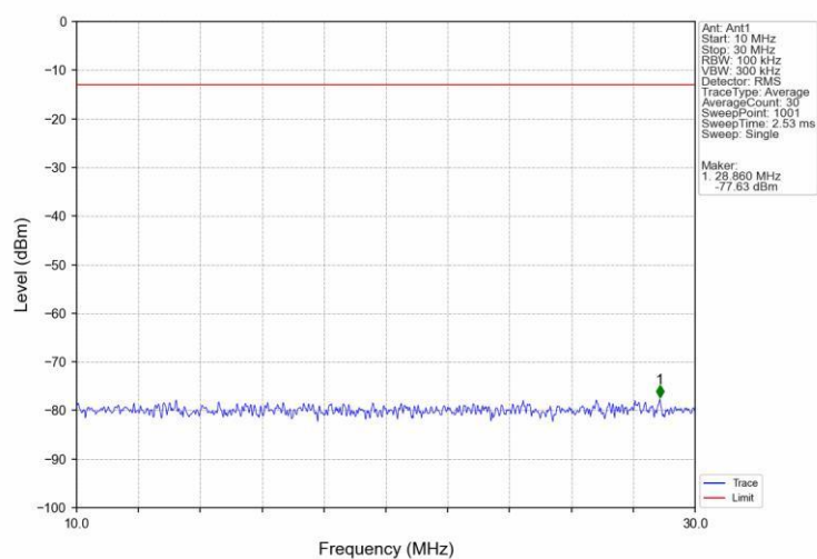
Band25_15MHz_QPSK_MCH_1882.5MHz_RB_1_0_NTNV
