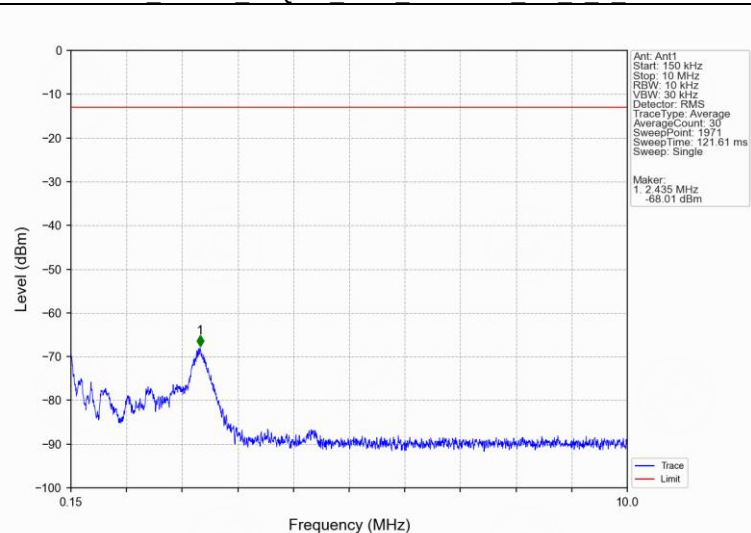
Band25_10MHz_16QAM_HCH_1910MHz_RB_1_0_NTNV
