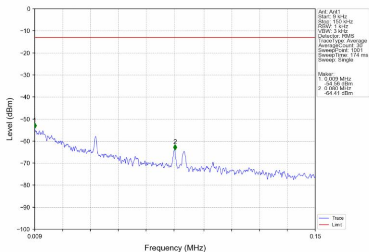
Band25_15MHz_16QAM_MCH_1882.5MHz_RB_1_0_NTNV
