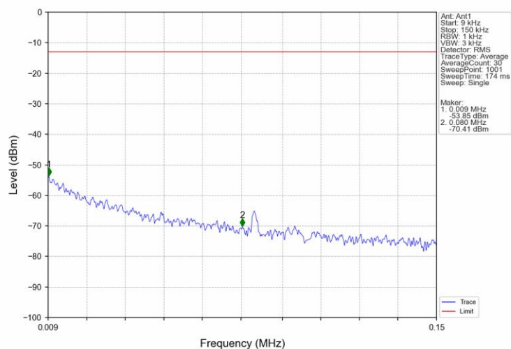
Band25_20MHz_16QAM_MCH_1882.5MHz_RB_1_0_NTNV
