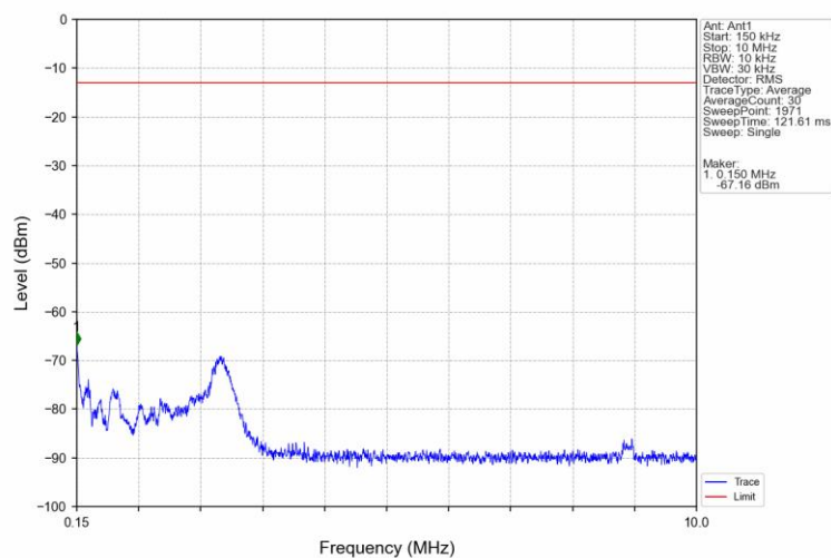
Band25_20MHz_16QAM_MCH_1882.5MHz_RB_1_0_NTNV
