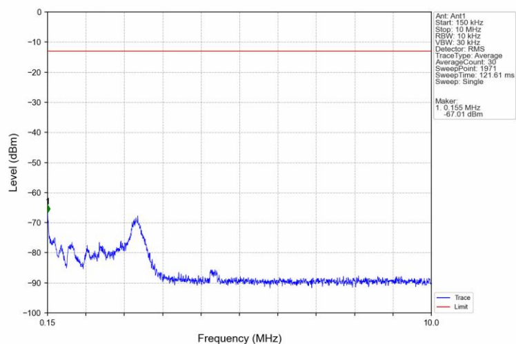
Band25_10MHz_QPSK_MCH_1882.5MHz_RB_1_0_NTNV
