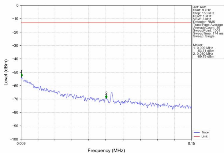
Band25_10MHz_16QAM_MCH_1882.5MHz_RB_1_0_NTNV
