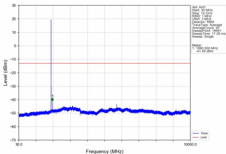
Band25 10MHz 16QAM HCH 1910MHz RB 1 0 NTV
