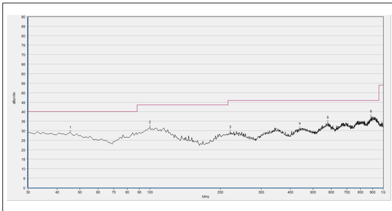
(30MHz – 1GHz, Test Antenna Vertical)
