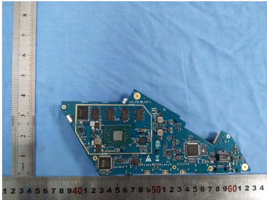
EUT - AJ3-V56-MB-V20-1 Board Uncovered View
