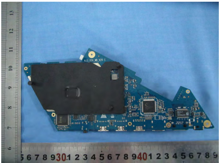
EUT - AJ3-V56-MB-V20-1 Board Top View
